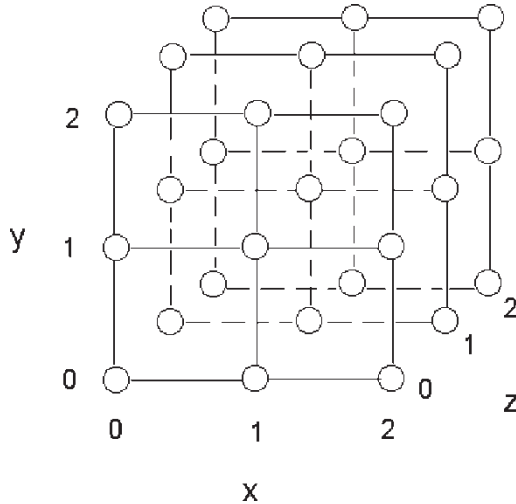
Figure 4. The calibration points in the virtual 3 \times 3 \times 3 cube. The PSOM computation uses a 3D coordinate system that maps every calibration point to the value 0, 1, or 2 in each dimension.
