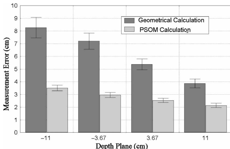
Figure 7. The measurement errors for the gaze-point calculation at different depth planes. The values on the x-axis indicate how far before (positive values) or behind (negative values) the corresponding depth plane is located relative to the screen plane. Error bars show standard error.
