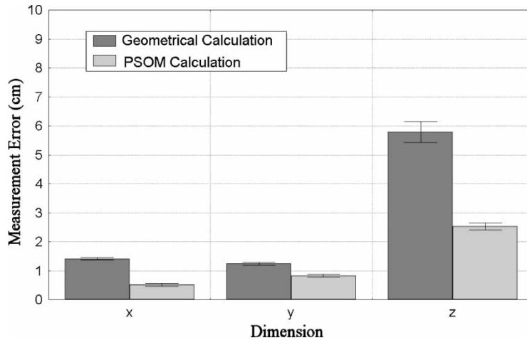
Figure 8. The measurement errors for the gaze-point calculation relating to the x -, y - and z -coordinates. Error bars show standard error.
