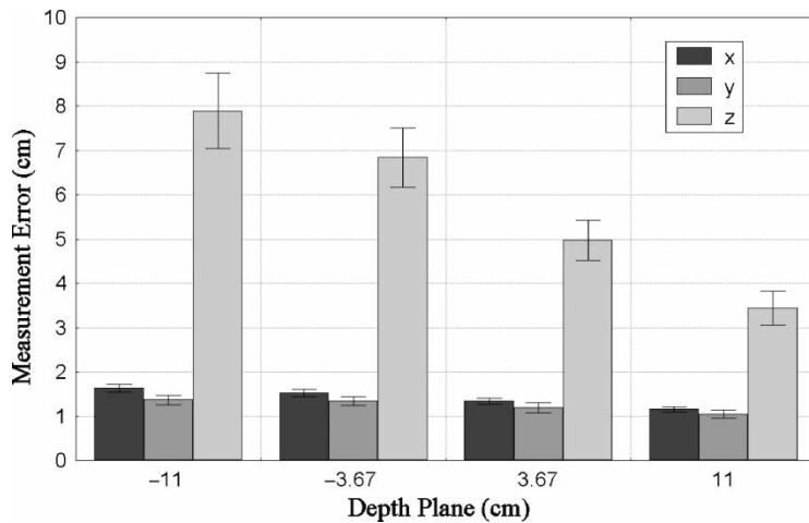
Figure 9. The measurement errors in the gaze-point calculation using the geometrical method. The values on the x-axis indicate how far before (positive values) or behind (negative values) the corresponding depth plane is located relative to the screen plane. Error bars show standard error.
