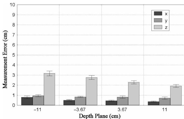
Figure 10. The measurement errors of the gaze point calculation using the neural network. The values on the x-axis indicate how far before (positive values) or behind (negative values) the corresponding depth plane is located relative to the screen plane. Error bars show standard error.
