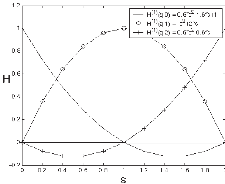
Figure 5. The three different basis functions.
