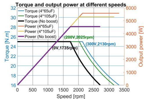
Fig. 10 Torque/speed and power/speed characteristics
