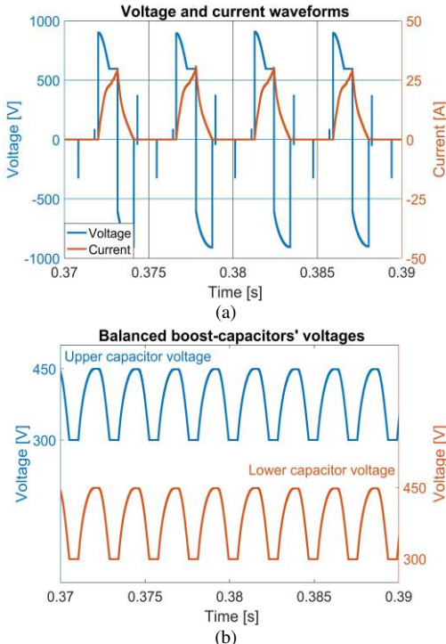
Fig. 8 SRM waveforms with 65\mu\text{F} boost-capacitors: (a) phase voltage and current at base speed and (b) boost-capacitors, C_U and C_L voltages.
