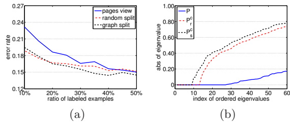
Figure 2. Result on the view split method. (a) The x -axis shows the amount of labeled examples (in the ratio of L ), and the y -axis shows the error rate; (b) the x -axis shows the index of the ascendingly ordered eigenvalues, and the y -axis shows the absolute value of the eigenvalues.
