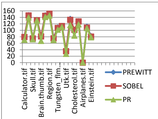
RMSE
