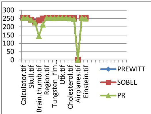
MD
