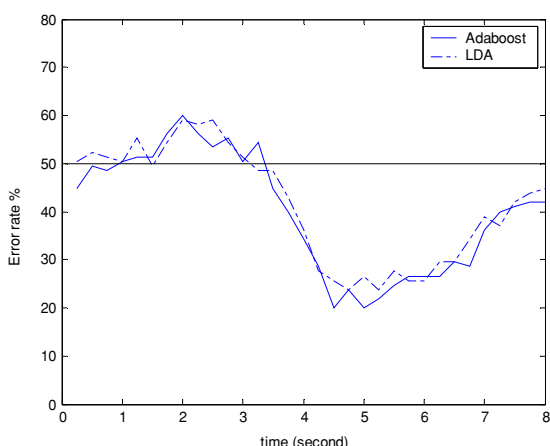
Figure 8. Error rate of FD with Adaboost and LDA for subject o8.
