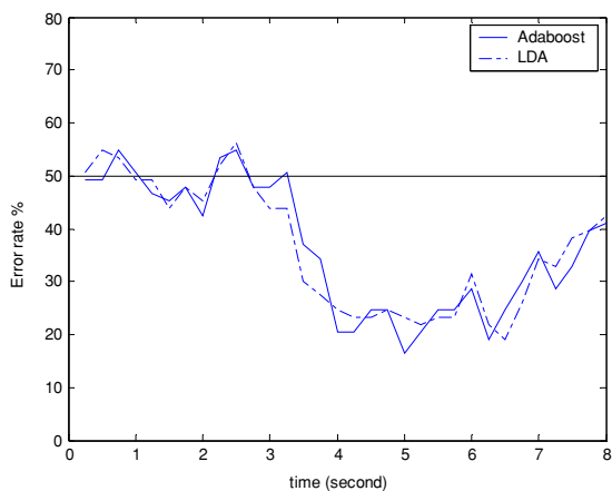
Figure 7. Error rate of FD with Adaboost and LDA for subject o3.
