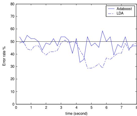
Figure 3. Error rate of BP with Adaboost and LDA for subject L1.
