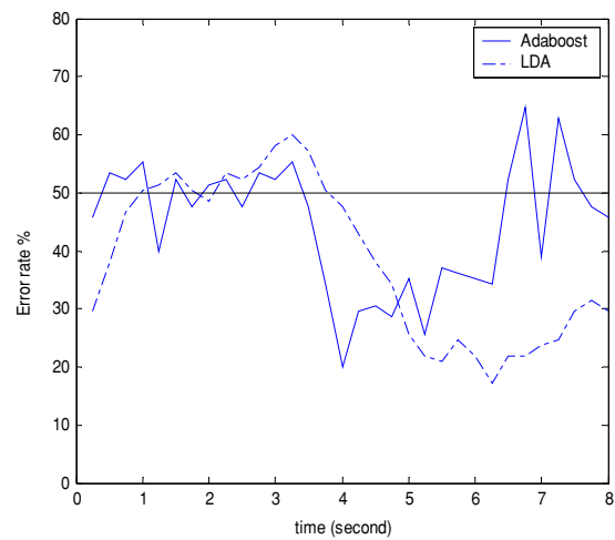
Figure 5. Error rate of BP with Adaboost and LDA for subject o8.
