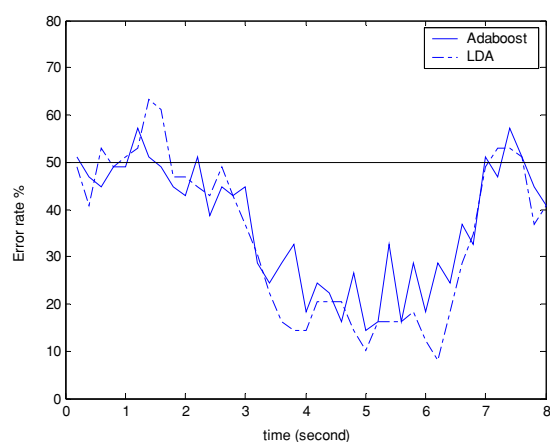
Figure 11. Error rate of FD with Adaboost and LDA for subject k3.
