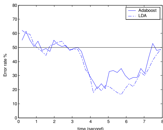
Figure 10. Error rate of BP with Adaboost and LDA for subject f8.
