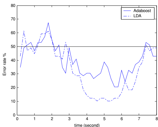
Figure 9. Error rate of BP with Adaboost and LDA for subject k3.
