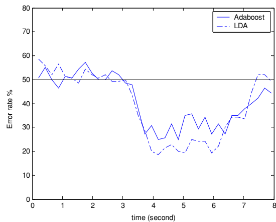
Figure 12. Error rate of FD with Adaboost and LDA for subject f8.
