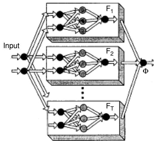
Figure 2. A committee of neural networks generated using Adaboost. F_1 , F_2 and F_T are the output of weak learners and the output \phi is the total output of the Adaboost [14].
