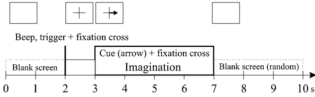
Figure 1. Training paradigm.
