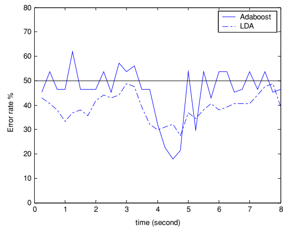
Figure 6. Error rate of FD with Adaboost and LDA for subject L1.
