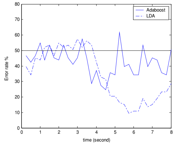
Figure 4. Error rate of BP with Adaboost and LDA for subject o3.
