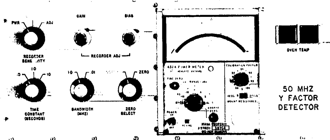
Fig. 3. Field model of power meter detector
