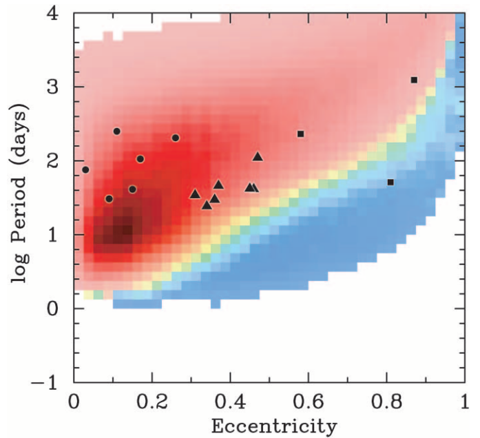
FIG. 5.—Distribution of orbital period and eccentricity for the systems in Fig. 4 with secondary masses greater than 8 M_{\odot} . A value of \sigma = 20 \text{ km s}^{-1} applied to the NSs born in all case B_e and C_e binaries and \sigma = 200 applied to all other NSs. The colors, intensities, and symbols have the same meaning as in Fig. 3.
