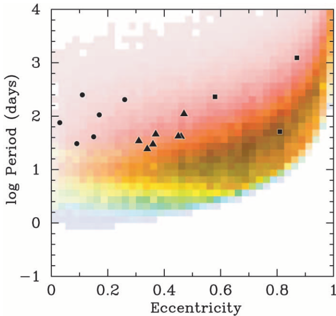
FIG. 3.—Two-dimensional distribution of orbital period and eccentricity for the systems in Fig. 2 with secondary masses greater than 8 M_{\odot} . The intensity and color of a given square “pixel” indicate the total number of binaries and the stability of mass transfer, respectively. Pure red indicates only stable mass transfer, while pure blue indicates only dynamically unstable mass transfer. Colors that are not blue or red represent a mixture of stable and unstable systems; pure green indicates equal numbers. The intensity scale is linear and the lightest pixels represent \sim 1\% of the number contained in the most intense pixel in the figure. Overlaid on the plot are markers that show the period and eccentricity (or upper limit) for the wide, low-eccentricity HMXBs ( circles ), the better known eccentric HMXBs ( triangles ), and the long-period binary radio pulsars with massive companions ( squares ). The short-period, nearly circular HMXBs have not been plotted.
