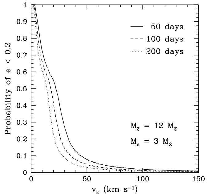
FIG. 1.—Probability that the post-SN eccentricity is less than 0.2 for a helium star of mass 3 M_{\odot} and a secondary of mass 12 M_{\odot} , for three different pre-SN orbital periods, as a function of the kick speed. The directions of the kicks are distributed isotropically.
