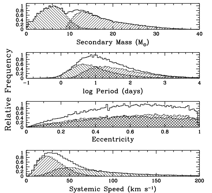
FIG. 2.—Distributions of binary parameters of systems that have undergone case B or C mass transfer from the original primary star to the secondary, have been left bound following the subsequent supernova explosion, and have not merged to form a Thorne-Zytkow object (see text). Hatched regions indicate systems that have undergone stable mass transfer ( +45^\circ ) and dynamically unstable mass transfer ( -45^\circ ). The histogram that encloses the hatched region is the sum of the distributions for stable and unstable systems. A single Maxwellian kick distribution with \sigma = 200 \text{ km s}^{-1} has been applied to all NSs.
