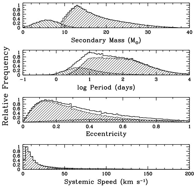
FIG. 4.—Same as Fig. 2, but with \sigma = 20 \text{ km s}^{-1} applied to the NSs born in all case B_e and C_e binaries and \sigma = 200 \text{ km s}^{-1} applied to all other NSs. Note that the eccentricity distribution for the stable systems has a distinct peak at e \sim 0.15 .
