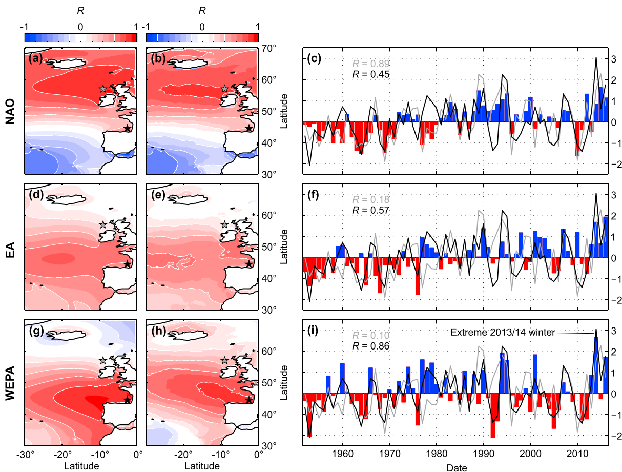
Figure 2. (a, b, d, e, g, and h) The spatial correlation of the winter (DJFM)-averaged H_s and H_{s95\%} , respectively, against the winter-averaged NAO (Figures 2a and 2b) and EA indices (Figures 2d and 2e), and against our new WEPA index (Figures 2g and 2h) computed as the normalized SLP difference measured between station Valentia (Ireland) and station Santa Cruz de Tenerife (Canary Islands, Spain). (c, f, and i) Time series of the corresponding indices with superimposed normalized winter-averaged H_s simulated at the buoys SC (Scotland, black) and BI (Biscay, grey) with corresponding correlation coefficient.
