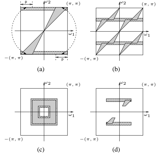
Fig. 3. Illustration of the frequency domain aliasing problem of the contourlet transform. Gray regions represent the ideal passband support. Patterned regions represent the aliasing components or transition bands. (a) One directional filter. (b) The directional filter after being upsampled by 2 along each dimension. (c) A bandpass filter from the Laplacian pyramid. (d) The resulting contourlet subband.
