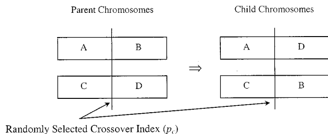
Fig. 6. Crossover operation.
