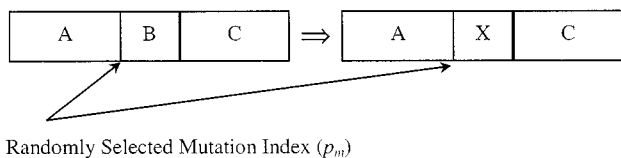
Fig. 5. Mutation operation.
