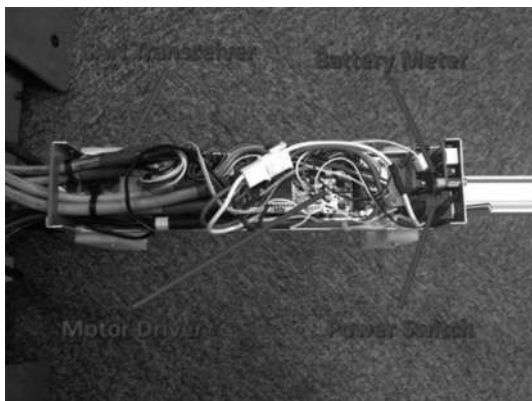
Fig. 10 Internal circuit
