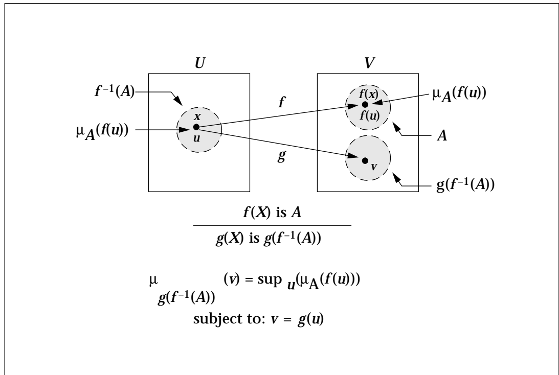
Figure 10. Schematic of the Generalized Extension Principle.
