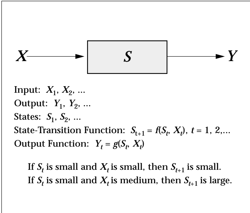
Figure 6. Perception-Based System Modeling.
