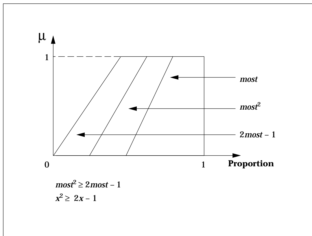
Figure 4. Membership Functions of "Most" and Related Perceptual (Fuzzy) Quantifiers.
