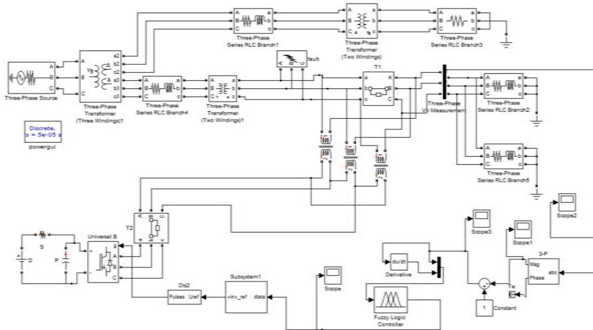
Fig. 9 Matlab/Simulink Power Circuit Model of DVR
