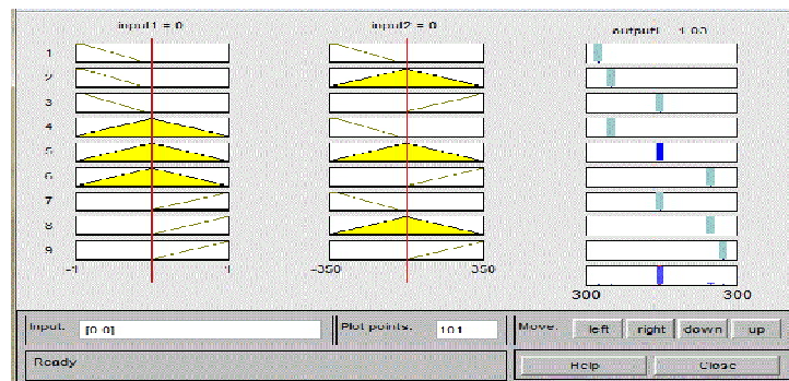
Fig. 8 Mamdani-type based rule viewer for controller
