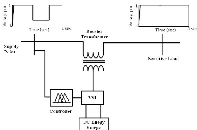
Fig. 1 Schematic diagram of DVR system
