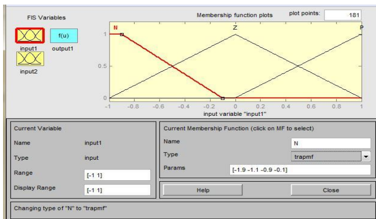
Fig. 3 Membership Function for Mamdan-type Fuzzy Logic Input Variable
