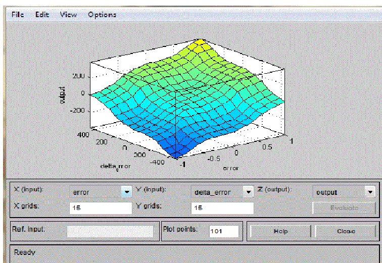
Fig. 10 Surface View Using Mamdani-type Fuzzy Logic Algorithm
