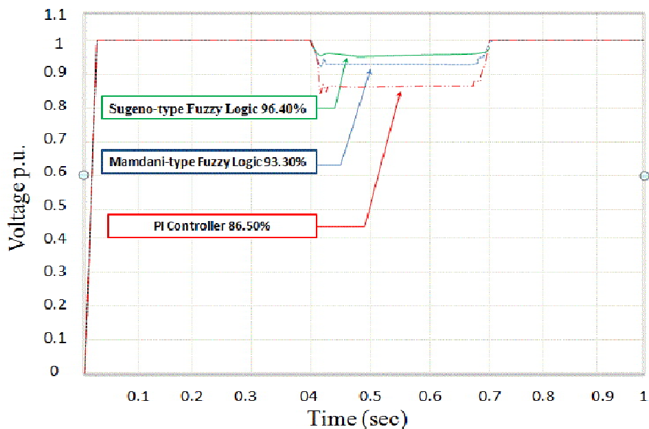
Fig. 13 (b) Two-Phase Comparison of Sugeno-Type Fuzzy Logic, Mamdani-Type Fuzzy Logic, and PI Controller
