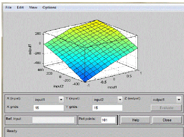
Fig. 11 Surface View Using Sugeno-type Fuzzy Logic Algorithm
