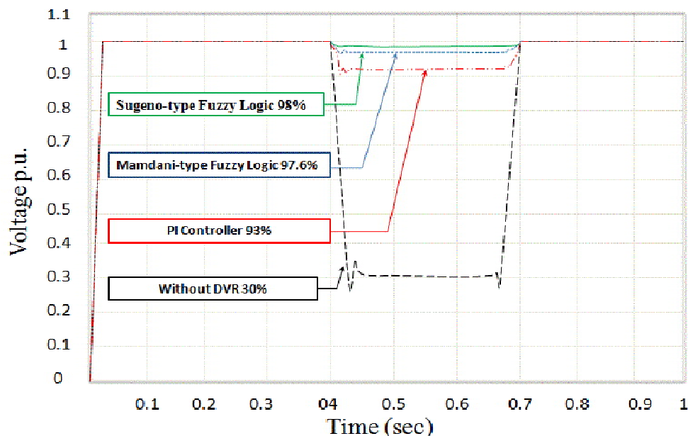
Fig. 12 (a) Single-Phase Comparison of Sugeno-Type Fuzzy Logic, Mamdani-Type Fuzzy Logic, PI Controller, and Without DVR
