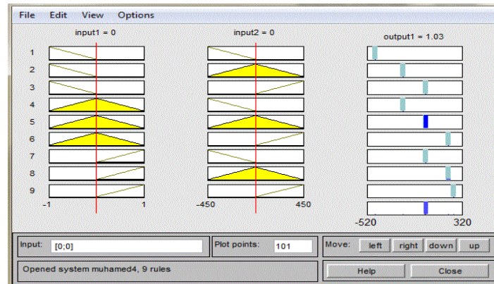
Fig. 9 Sugeno-type based rule viewer for controller
