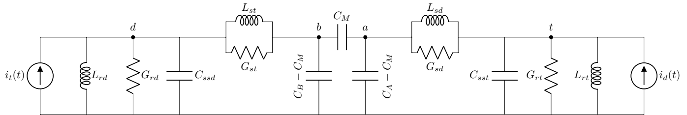
Figure 6: Equivalent circuit for half-car using $\Pi$-network model.
