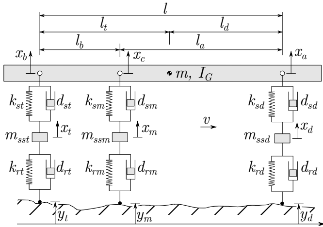
Figure 7: Three-axle vehicle model for vertical dynamics analysis.
