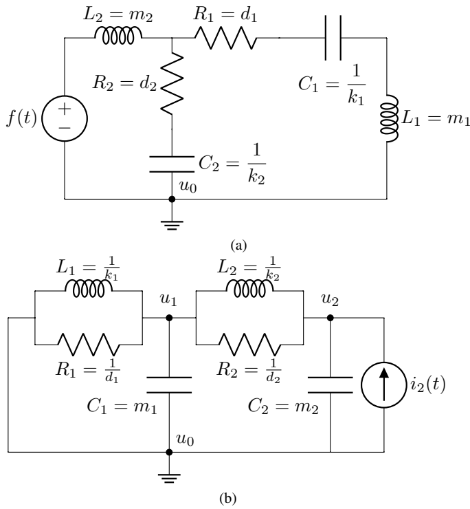
Figure 2: (a) Force-voltage and (b) force-current analogues of the 2 d.o.f. mechanical model of figure 1.
