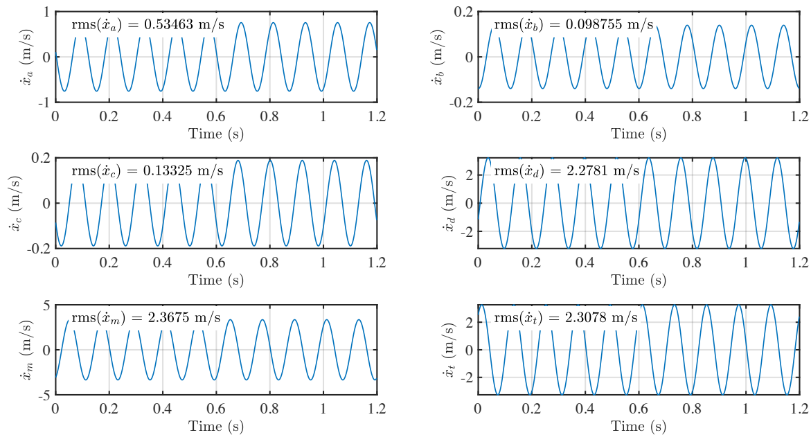
Figure 9: Steady state vertical oscillation velocities of the characteristic points ( a , b , c , d , m , and t ) of the three-axle vehicle model.
