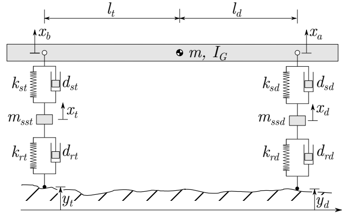
Figure 3: Half-car vehicle model for vertical dynamics analysis.
