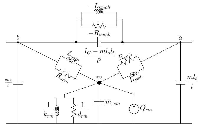
Figure 8: Electrical analogue of the three-axle vehicle model (zoomed in the coupling area of figure 6). L_{sma} = \frac{l}{k_{sm} l_a} , L_{smb} = \frac{l}{k_{sm} l_b} , R_{sma} = \frac{l}{R_{sm} l_a} , R_{smb} = \frac{l}{k_{sm} l_b} , L_{smab} = \frac{l}{k_{sm} l_a l_b} and R_{smab} = \frac{l}{R_{sm} l_a l_b}
