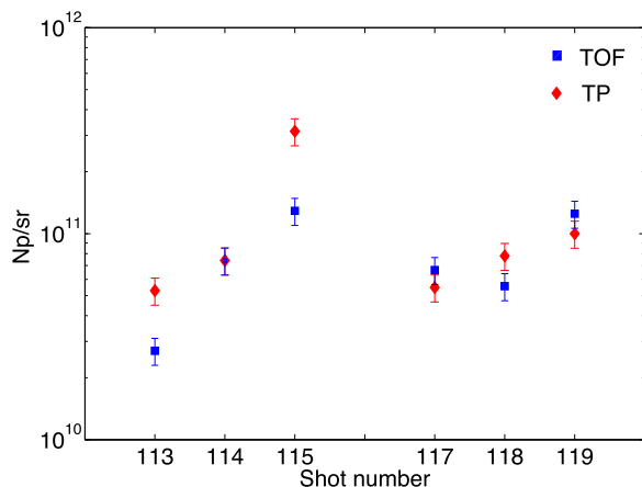
FIG. 8. Number of protons per solid angle in the energy range 13–18 MeV reconstructed with TOF technique (blue solid squares) and TPS images (red solid diamonds) for 6 consecutive shots.
