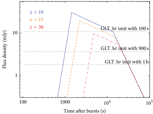
FIGURE 9: Expected light curves of GRB afterglows at z = 10, 15, and 30 at 230 GHz. Other physical parameters are fixed as E = 1 \times 10^{53} , \Gamma = 80 , n = 1 , \epsilon_e = 0.3 , \epsilon_{B,RS} = 0.03 , and \epsilon_{B,FS} = 0.01 . The expected GLT 3\text{-}\sigma limits with 900 s and 1 h exposure are indicated with dotted lines. GLT with rapid follow-ups has sufficient potential to detect these higher- z events.
