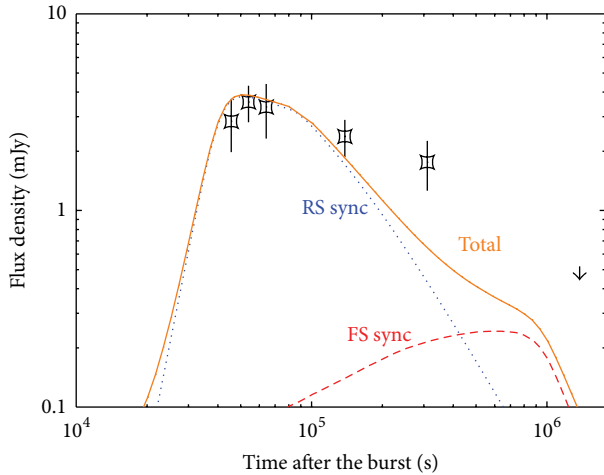
FIGURE 4: Submm light curve of GRB120326A with RS and FS model functions.
