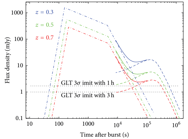
FIGURE 8: Expected RS (dashed-dot) and FS (dashed) light curves in the 230 GHz band at z = 0.3, 0.5 , and 0.7 with E = 3 \times 10^{52} erg, n = 1 \text{ cm}^{-3} , p = 2.1 , \epsilon_e = 0.3 , and \epsilon_{B,FS} = 0.01 . Solid lines indicate the total of RS and FS. GLT has also enough sensitivity to characterize the FS components for nearby ( z \lesssim 0.7 ) GRBs. The expected GLT 3- \sigma limits with 1 h and 3 h exposure are indicated with dotted lines.
