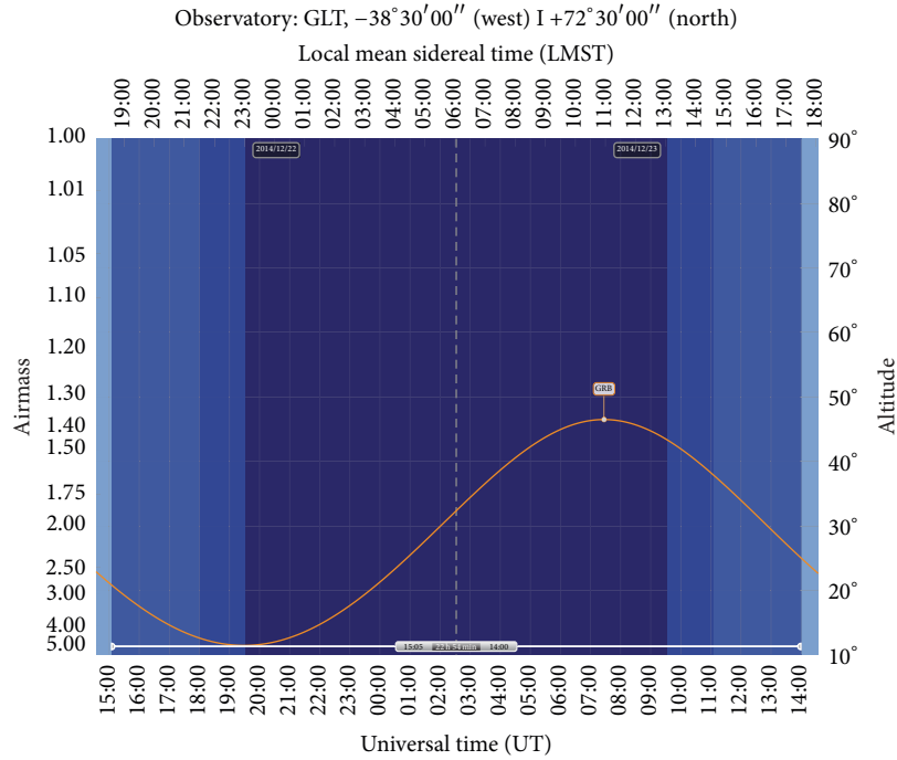
FIGURE 5: An example of visibility plot in winter for the GRB that declination is 29 deg. Hatches indicate the sun altitude lower than -18 (dark blue), -12 (blue), -6 (dark cyan), and 0 (cyan) deg., respectively.
