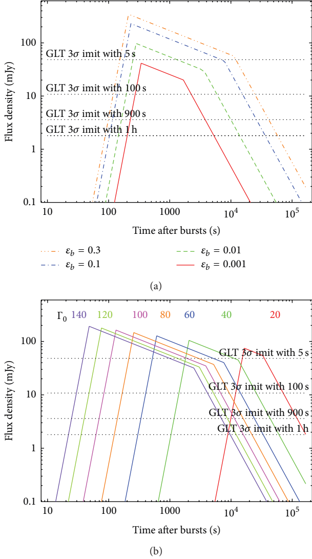
FIGURE 6: (a) Expected RS light curves in the 230 GHz band with various \epsilon_{B,RS} (0.001, 0.01, 0.1, and 0.3). Other physical parameters are fixed as z = 1 , E = 3 \times 10^{52} , \Gamma = 80 , n = 1 , \epsilon_e = 0.3 , and \epsilon_{B,FS} = 0.01 . (b) Expected RS light curves in the 230 GHz band with various initial Lorentz factor \Gamma_0 . Other physical parameters are z = 1 , E = 3 \times 10^{52} , n = 1 , \epsilon_e = 0.3 , \epsilon_{B,RS} = 0.03 , and \epsilon_{B,FS} = 0.01 . The expected GLT 3- \sigma limits with 900 s and 1 h exposure are indicated with dotted lines in both panels.
