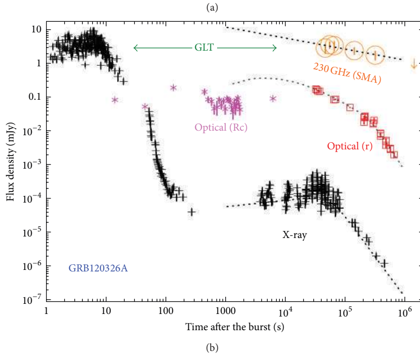
FIGURE 1: (a) Schematic summary of the GRB observational achievements along with time from the bursts in individual wavelength (from \gamma -ray to submm). (b) One of actual light curves in X-ray, optical, and submm with the earliest submm detection.
