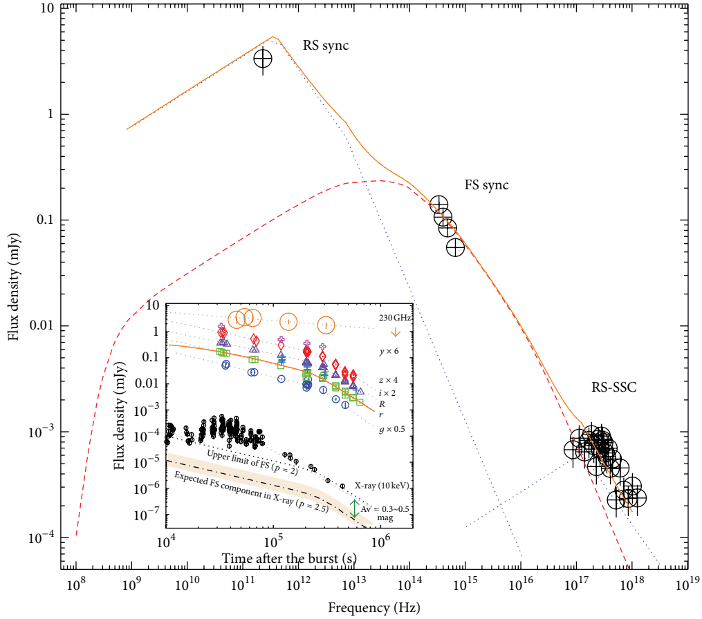
FIGURE 3: Main panel: The spectral energy distribution of GRB120326A at 6.42 \times 10^4 s after the burst [18]. The red dashed line shows the forward shock synchrotron model spectrum calculated using the boxfit code [89] with the same parameters for the best modeling light curve shown in the subpanel. The blue dotted lines show the reverse shock synchrotron radiation and its self-inverse Compton component calculated based on Kobayashi et al. [72] using the observed values and model function for the forward shock component. Subpanel: X-ray, optical, and submm light curves of the GRB120326A afterglow. The grey dotted lines show the best analytical fitted functions described in the text. The orange solid line shows the best modeling function for the r -band light curve obtained with the numerical simulation using boxfit.
