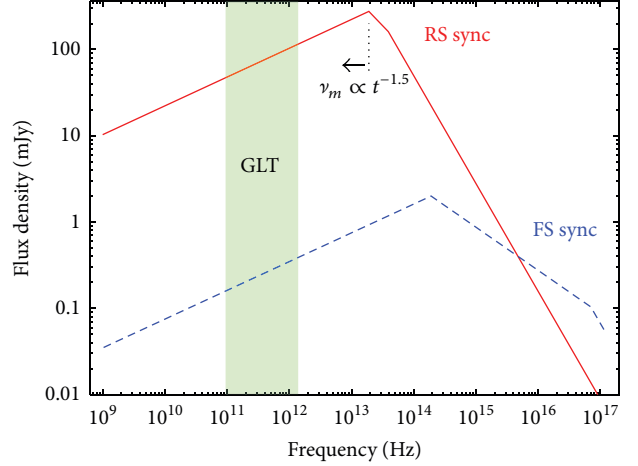
FIGURE 7: Expected spectrum at the deceleration time with z = 1 , E = 1 \times 10^{52} , \Gamma = 80 , n = 1 , \epsilon_e = 0.3 , \epsilon_{B,RS} = 0.03 , and \epsilon_{B,FS} = 0.01 . Synchrotron radiations from reverse and forward shock are indicated by red solid and blue dashed lines, respectively. A green hatched box indicates the frequency coverage of GLT.
