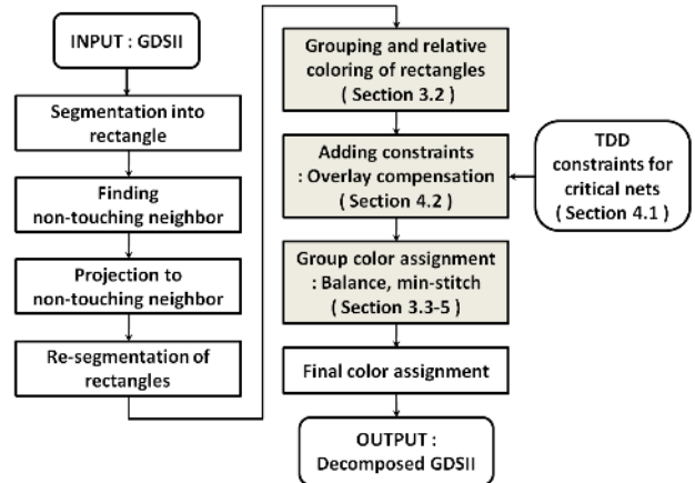
Figure 4: Overall flow of the decomposition framework.
