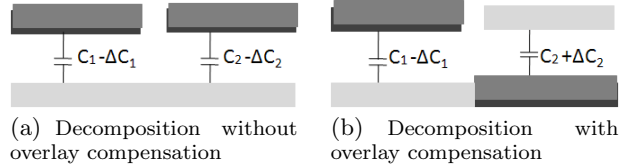
Figure 3: Overlay compensated decomposition.
