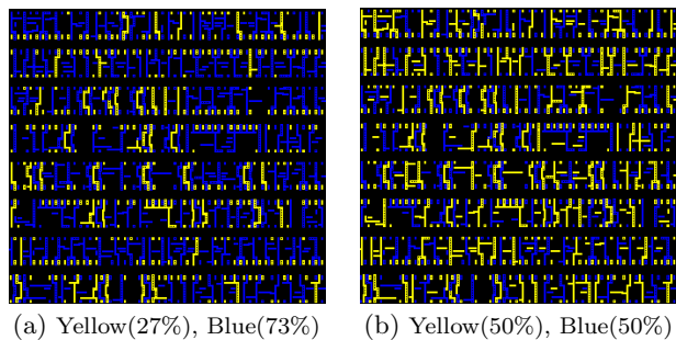
Figure 13: C432 decomposed layout.
