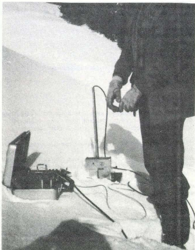
Fig. 4. The DTR in use in the field. The control unit is in the foreground, and the probe has just been inserted into about 1.6 m of snow cover.
