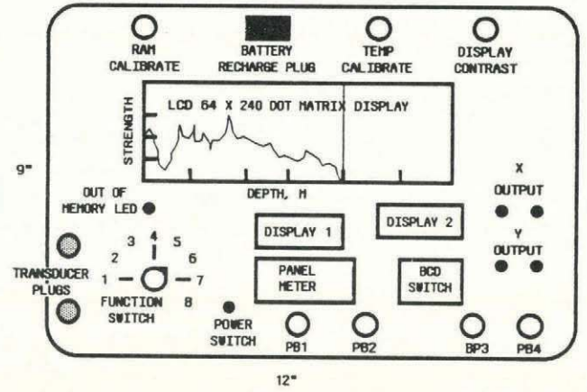
Fig. 3. Control unit lay-out for the DTR.
