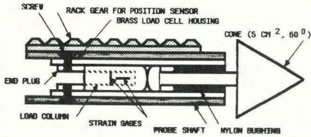
Fig. 1. Schematic of DTR probe showing the cone and load column with semi-conductor strain gages.
