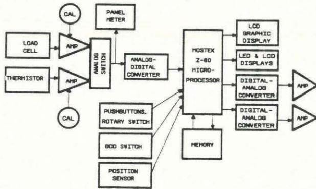
Fig. 2. Block diagram for the Digital Thermo-Resistograph.
