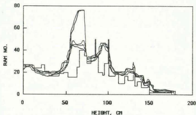
Fig. 5. Comparison of a number of DTR profiles with a ramsonde profile. The smooth curve is from the DTR.
