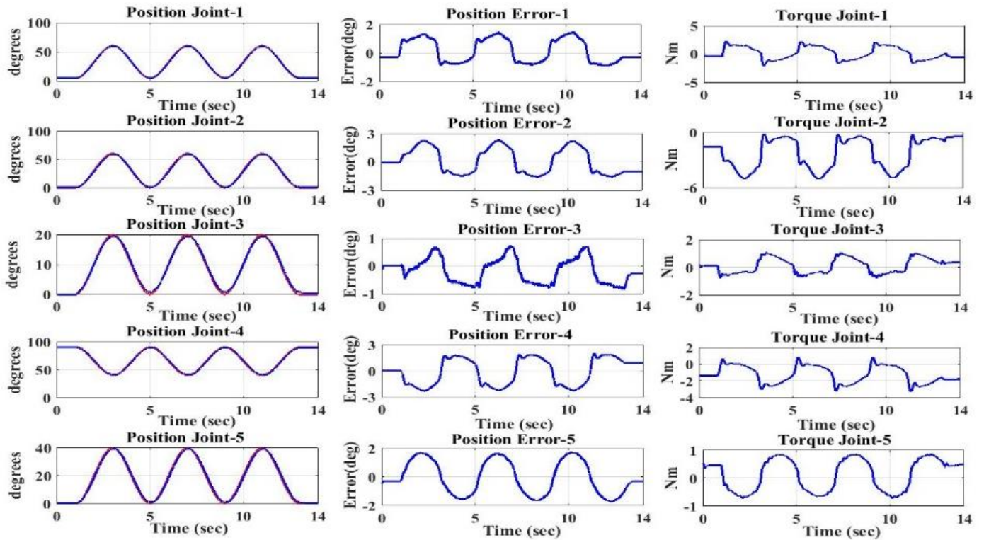
Fig. 2: Performance of the ETS-MARSE robot with subject-A in joint space.
