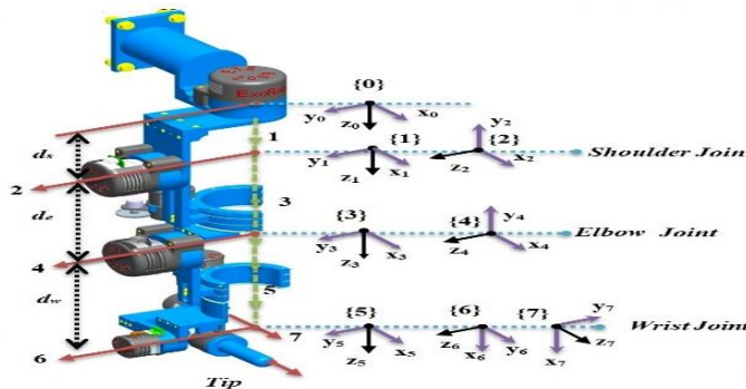
Fig. 1: Reference frames of ETS-MARSE.
