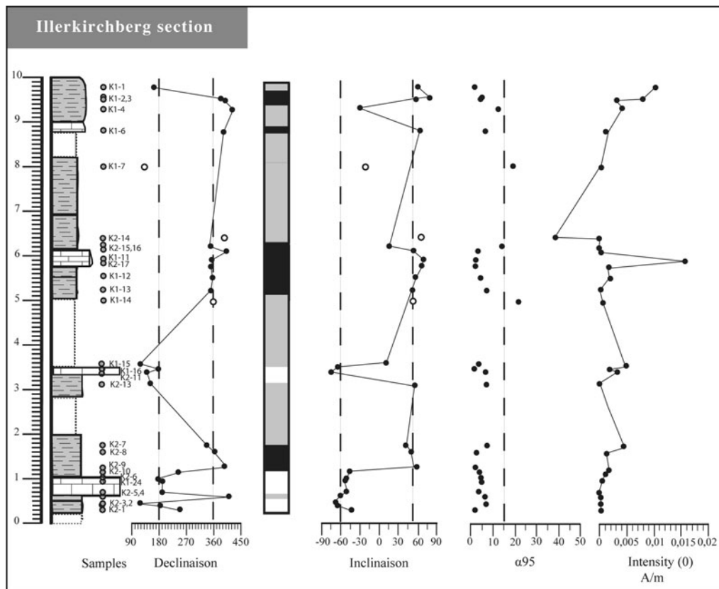
Fig. 9 Palaeomagnetic results of the Illerkirchberg section. For details see caption of Fig. 8
