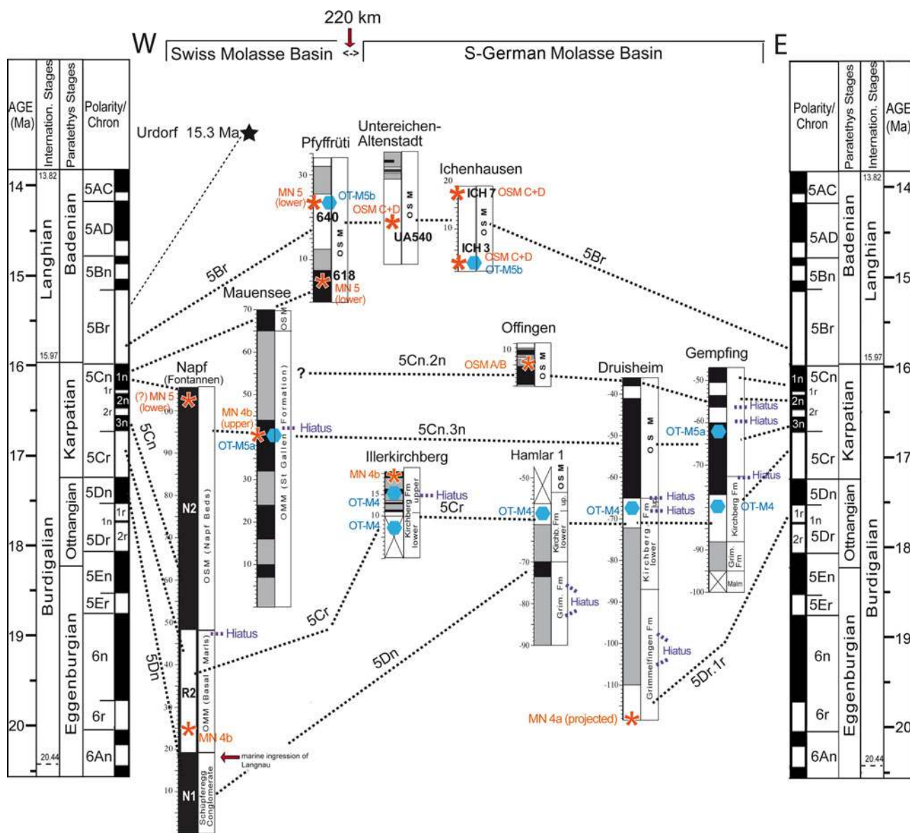
Fig. 12 Interpretation of the magnetostratigraphy of the Upper Marine Molasse (OMM), Upper Brackish Molasse (OBM), and Upper Freshwater Molasse (OSM) in the Swiss and S-German Molasse Basin; polarity pattern of the Napf section according to Kälin and Kempf (2009), polarity pattern of the sections Untereichen-Altenstadt, Ichenhausen and Offingen according to Abdul Aziz et al.
