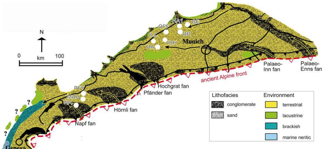
Fig. 3 Palaeogeographic situation at the time period of the Upper Freshwater Molasse (older part) and position of the sections that are important for this study. NA, Napf (Kälin and Kempf 2009); MAU, Mauensee (this study); PFY, Schmiedrued-Pfyffrüti and Schmiedrued-Dorfbach (this study); ILL, Iller Kirchberg (this study); UA,
