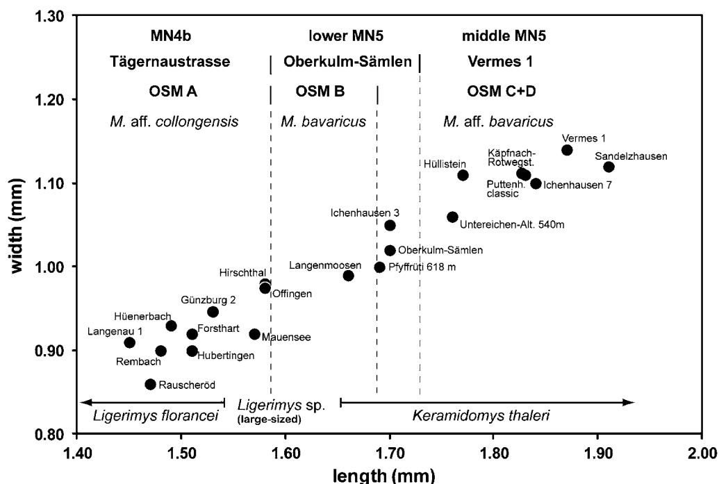
Fig. 11 Length–width diagram of the first lower molar (mean values) of cricetids representing the Megacricetodon evolutionary lineage from sites in the Swiss and S-German Molasse Basin. Note that the evolution of the lineage is mainly characterized by increase in molar length. The last occurrences of the eomyids Ligerimys florancei and Ligerimys sp. and the first occurrence of Keramidomys thaleri determine the “boundary” between the mammal units MN 4b and MN 5. Data for Günzburg 2 (n = 13) refer to measurements made by JP (this study) and data for Käpfnach-Rotwegstollen (n = 5) and Schmiedrueid-Pfyfrützbach 618 m (n = 5) were conducted by DK
