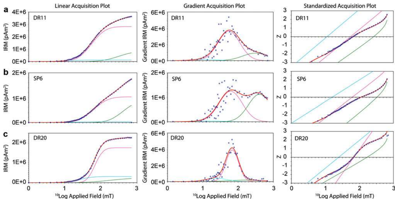
Fig. 6 Representative examples of the IRM component analysis (Kruiver et al. 2001). a Druisheim core: wide DP typical for detrital magnetite. b Pfyffrütli section: two components, detrital magnetite and hematite. c Druisheim core: narrow DP (0.2) typical for biogenic magnetite
