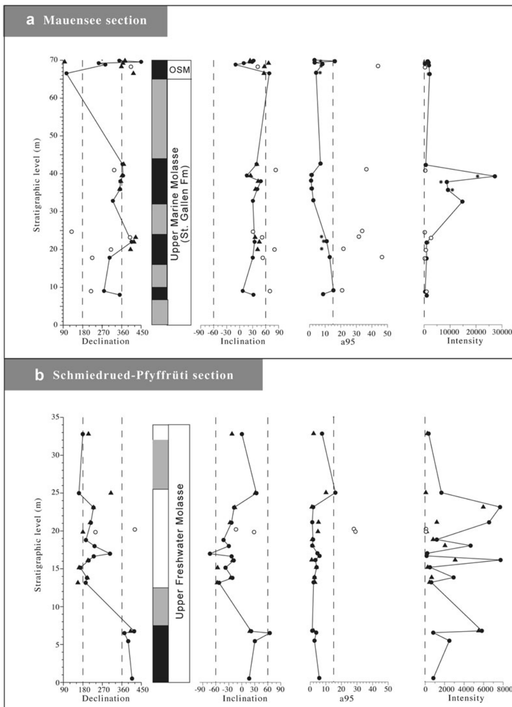
Fig. 8 Palaeomagnetic results of the Mauensee (a) and Schmiedrued-Pfyffrüti (b) sections. The black dots (triangles) in the declination, inclination and a95 records represent reliable ChRM directions after thermal (alternating field) demagnetisation, the white dots (triangles)
