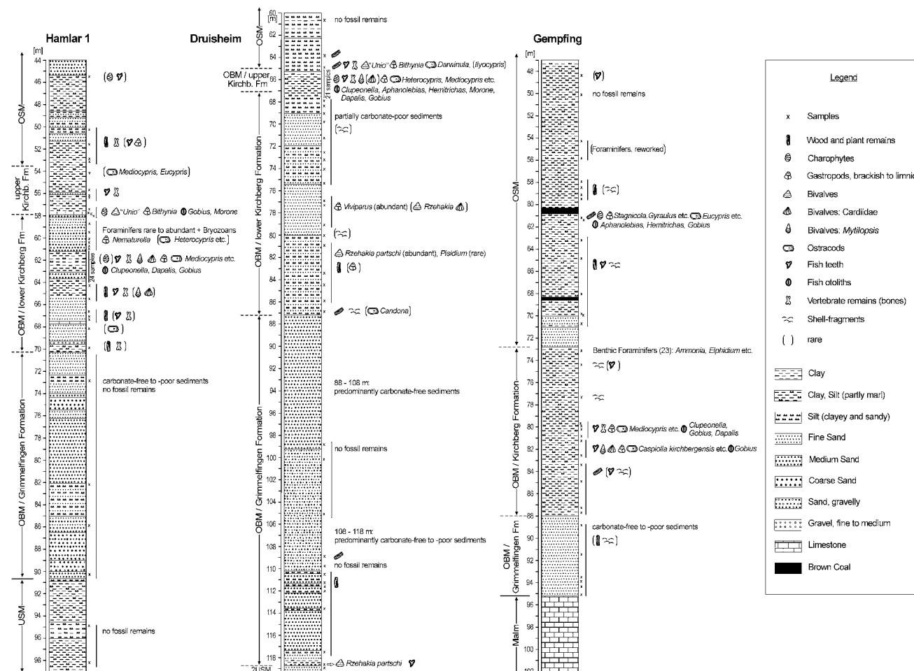
Fig. 5 Lithostratigraphy, lithology and fossil content of the studied boreholes
