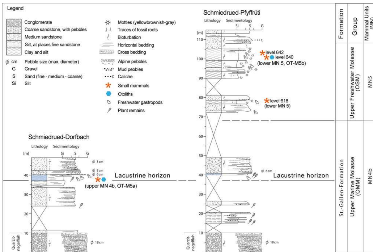
Fig. 4 Lithostratigraphy and lithofacies of the Schriedued-Dorfbach and Schriedued-Pfyfrüti sections. Modified from Graf et al. (2012)
