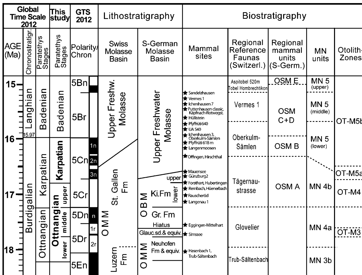
Fig. 13 New magnetostratigraphic framework and biostratigraphic correlation in the Swiss and S-German Molasse Basin and possible shift of the Ottnangian-Karpatian boundary (GTS according to Lourens et al. 2004; Gradstein et al. 2012). Note that the position of the MN4b/MN5 “boundary” varies, depending if it is set at the last occurrence of Ligerimys sp. or the last occurrence of Ligerimys florancei (see also Fig. 11). Note also that the correlation between the
