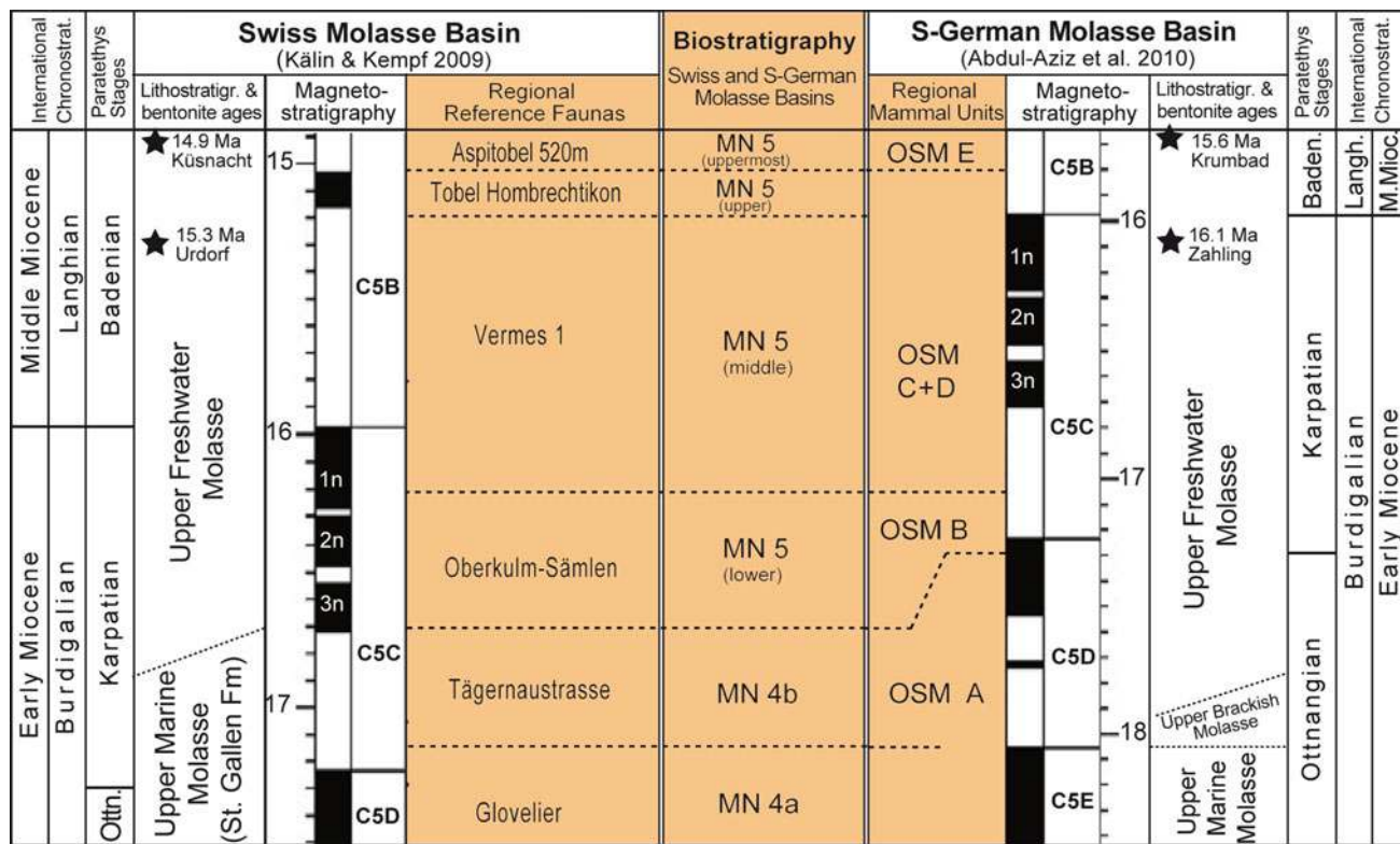
Fig. 1 Magnetostratigraphic and biostratigraphic framework in the Swiss and S-German Molasse Basin according to Kälin and Kempf (2009) (left columns) and Abdul Aziz et al. (2010) (right columns). Note the great difference between the Swiss and S-German Molasse Basin in the correlation of the magnetostratigraphic records to the Global Time Scale (GTS), despite the biostratigraphy (coloured) indicate similar ages for these deposits. Correlation between the small
