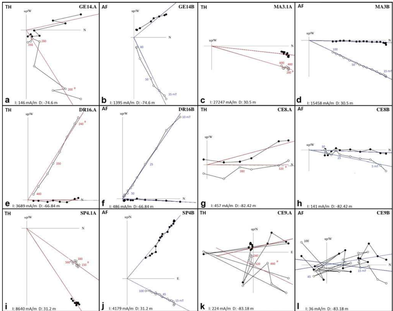
Fig. 7 Thermal (TH/red) and alternating field (AF/blue) demagnetization diagrams of characteristic samples. Values along the vectors are given in °C (TH) or mT (AF). I, intensity at 280° or at 35 mT; D,
