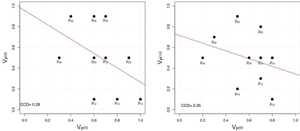
Figure 8: Plots of essential vectors of intensities of preferences corresponding to patients diagnosed Bipolar disorder versus OCD (Subsection 6.2) and the best adjusted line.
