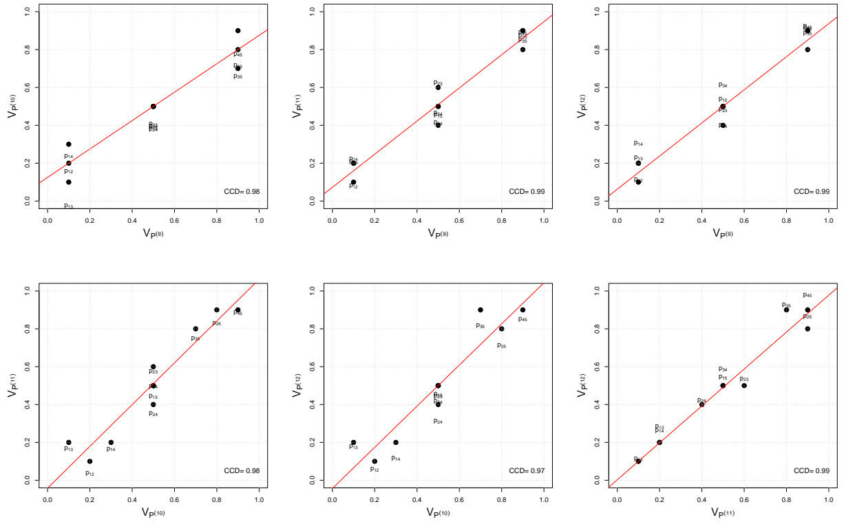
Figure 5: Plots of essential vectors of intensities of preferences corresponding to patients diagnosed OCD (Subsection 6.2) and the best adjusted line.
