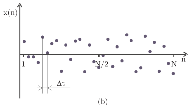
Fig. 4. Illustration of the idea of the NSP method for inherent noise signal which contains only RTS noise: (a) – noise signal, (b) – sampled signal data, (c) – data in XY plane
