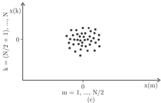
Fig. 3. Illustration of the NSP method results for a noise signal containing only Gaussian noise (without RTS noise), (a) – noise signal, (b) – sampled signal data, (c) – data in XY plane, \Delta t = 1/f_s sample period, the reciprocal of the sampling frequency
