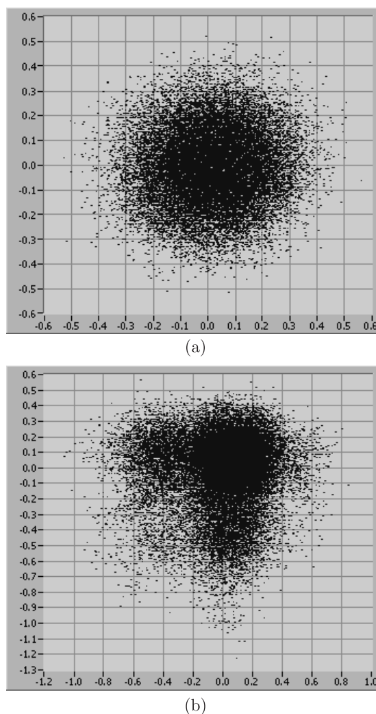
Fig. 6. NSP patterns for the inherent noise of two OCDs: (a) – Gaussian noise, (b) – Gaussian and RTS noise (after Ref. 1)
