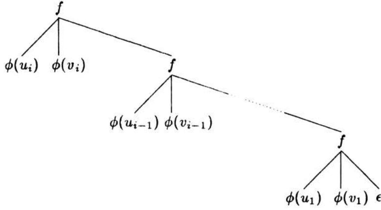
Figure 2: The term \psi((u_j, v_j)_{j=1\dots n})(i) representing the subsequence (u_j, v_j)_{j=1\dots i} of the sequence (u_j, v_j)_{j=1\dots n} for 1 \leq i \leq n
