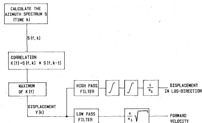
Fig. 3. Block diagram of reflectivity displacement method.
