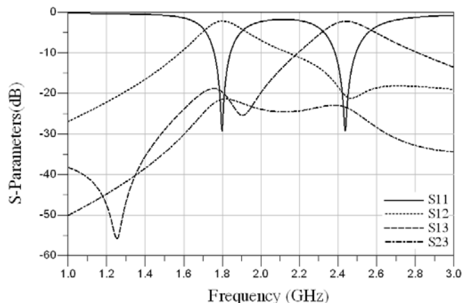
Fig. 5 Simulated frequency response of the proposed diplexer with ADS Agilent
