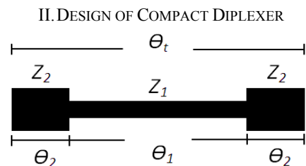
Fig. 1 Structure of the stepped impedance resonator (SIR)
