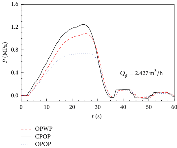
FIGURE 11: Surge pressure variation at different scenarios.
