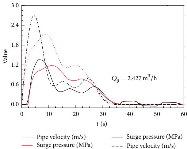
FIGURE 21: Surge pressure variations at different pipe velocities (gas influx Q_g = 2.427 \text{ m}^3/\text{h} ).
