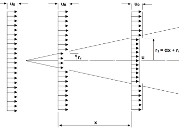
Fig.3 Wake Loss Model [2,3]
