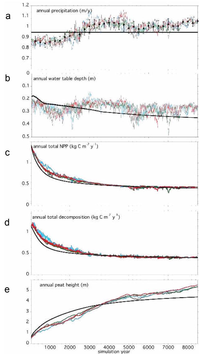
Fig. 4. (a) Four manifestations of annual precipitation ( \text{m y}^{-1} ) with amplitude of random variability \alpha = 2.5 and persistence \phi = 0.99 (see Eqs. 19–20). Solid black circles are regional mean annual precipitation at 250-year intervals, bars are regional variance, as determined by Muller et al. (2003b); solid black line represents constant mean annual precipitation. (b) HPM simulated annual water table depth (m below peat surface) for 4 random precipitation drivers and constant precipitation (solid black line). (c) Simulated annual total NPP for 4 random precipitation drivers and constant precipitation (solid black line). (d) Simulated annual total decomposition for 4 random precipitation drivers and constant precipitation (solid black line). (e) Simulated annual peat height for 4 random precipitation drivers and constant precipitation (solid black line). NOTE: all panels start with simulation year 50, avoiding the peatland initialization period (see text).
