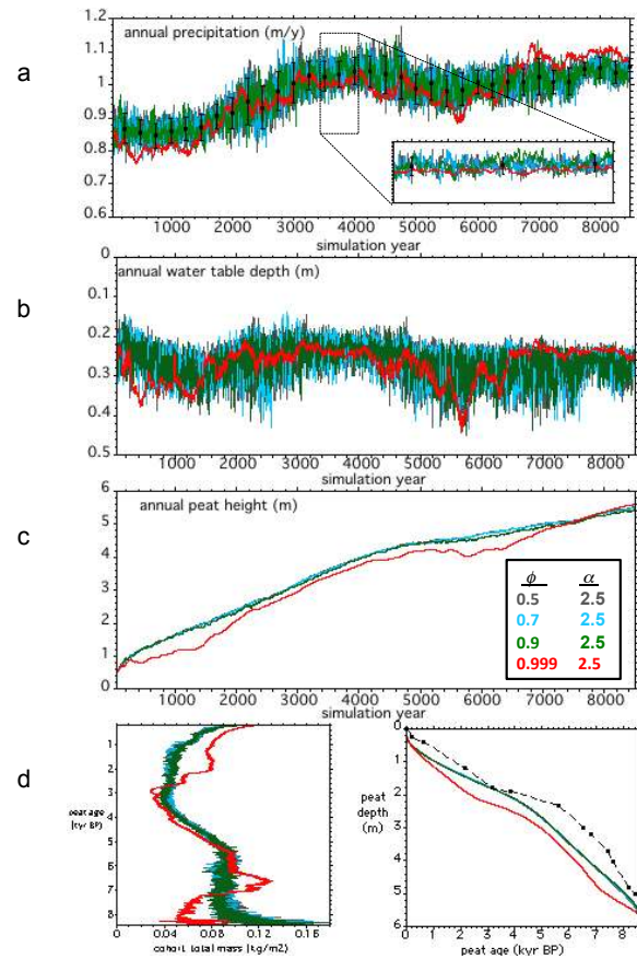
Fig. 8. Same as Fig. 7, but for simulations with \alpha=2.5 , and with \phi=0.5 (dark gray), 0.7 (cyan), 0.9 (green), and 0.999 (red) (see text and Eqs. 19, 20). In base runs (Figs. 4–6) \phi=0.99 .
