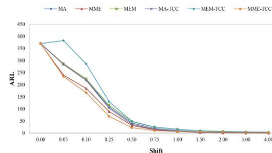
FIGURE 4. ARL curves of MA, MME, MEM, MA-TCC, MEM-TCC and MME-TCC control charts at ARL_0 = 370 , w = 5 and \lambda = 0.25 for gamma distribution.
