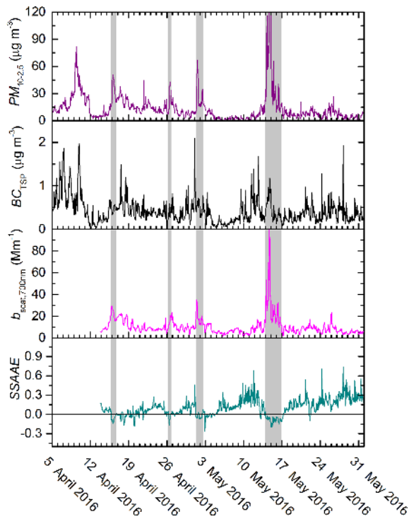
Figure 2. Time series of the mass concentration of coarse particles ( \text{PM}_{10-2.5} ) obtained by TEOM-FDMS, black carbon concentration (BC) for total suspended particles (TSP) obtained by AE33 Aethalometer, the light scattering coefficient at 700 nm obtained by nephelometer, and single scattering albedo Ångström exponent (SSAAE). The four periods with negative SSAAE during the campaign are shadowed.
