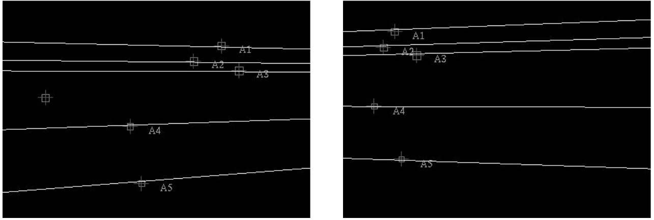
Fig. 3. Pair of stereo images during tracking process. Several retroreflective markers are tracked by the system. The crosses indicate the current blob position, while the frames quantify their size in the image. The labels A_i denote the corresponding points which minimize the epipolar constraint (white lines).
