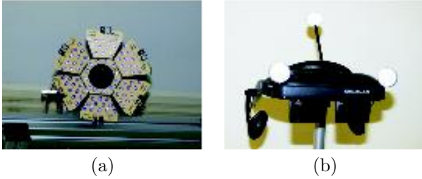
Fig. 2. (a) Closeup view of a camera with mounted IR lighting and IR filter. (b) See through head-mounted display with retroreflective markers.
