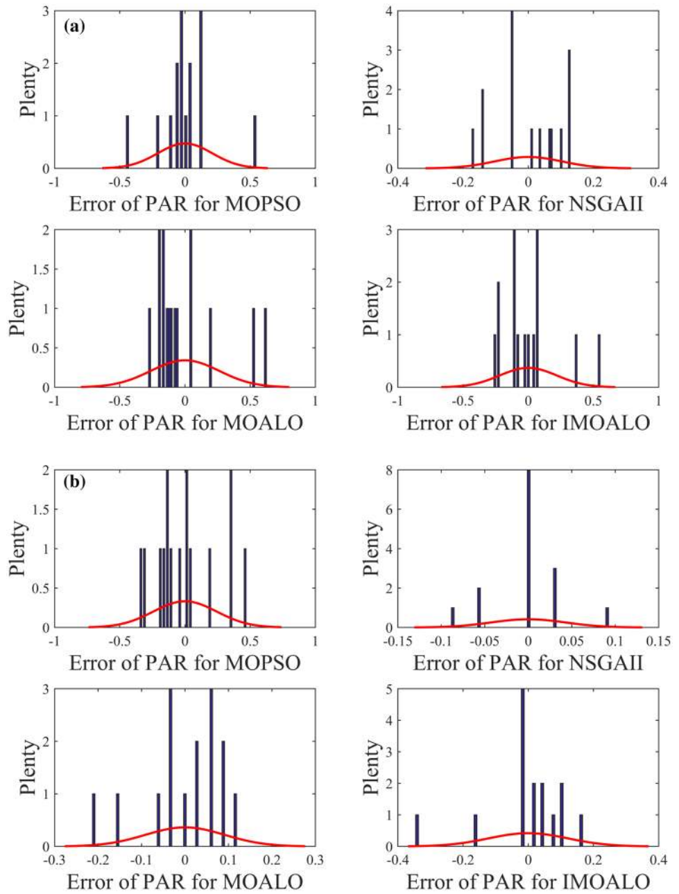
Fig. 8 Histogram plot for PAR a with an RTP signal b with CPP signal
