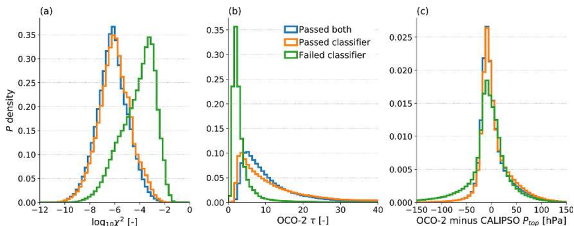
Figure 7. Normalised histograms of OCO2CLD-LIDAR-AUX outputs where SZA < 45°, separated into whether the soundings pass the new pre-processor flag and retrieval or not. The “passed both” set are those that returned valid cloud properties from the LUT along with T_{\text{top}} > 0^{\circ}\text{C} ; the “passed-classifier” case gave invalid cloud values or had T_{\text{top}} < 0^{\circ}\text{C} ; and the “failed-classifier” set are those that were attempted in OCO2CLD-LIDAR-AUX but are not passed by the new classifier. (a) Logarithm of \chi^2 ; (b) retrieved \tau ; (c) P_{\text{top}} minus the closest CALIPSO retrieved P_{\text{top}} .
