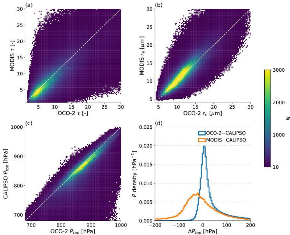
Figure 5. Inter-satellite comparison of retrieved cloud properties of (a) MODIS vs. OCO-2 \tau , (b) MODIS vs. OCO-2 r_e , (c) CALIPSO vs. OCO-2 P_{top} , and (d) OCO-2 or MODIS P_{top} minus CALIPSO P_{top} . The colour bar on the right applies to (a, b, c).
