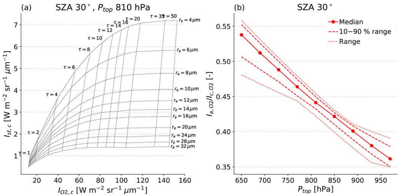
Figure 4. Example lookup table (LUT) properties. (a) Radiance in the strong CO 2 continuum as a function of A-band continuum radiance at SZA = 30° for clouds with P_{top} = 810 hPa and \tau and r_e as labelled. (b) A-band absorption ratio within the SZA = 30° table as a function of P_{top} . The solid line is the median value within each LUT at a fixed P_{top} ; the dashed lines span the 10%–90% range, and the dotted lines span the minimum to maximum values.
