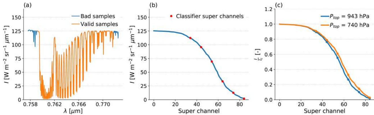
Figure 1. (a) OCO-2 A-band spectrum for a cloud with CALIPSO P_{\text{top}} = 943 hPa, with the used channels in orange and non-used (e.g. due to FPA pixel damage) in blue. (b) The smoothed super-channel spectrum, where the channels are ranked in brightness and then non-overlapping 10-channel means are taken. The super channels used in the classifier are shown in red. (c) Comparison of the ranked ratio I/I_c between this cloud, and one at a higher altitude ( P_{\text{top}} = 740 hPa). The SZA is within 0.01^\circ , and the continuum radiance is within 1 % between each spectrum; the differences are largely due to the shorter path length resulting in less absorption for the higher-altitude cloud.
