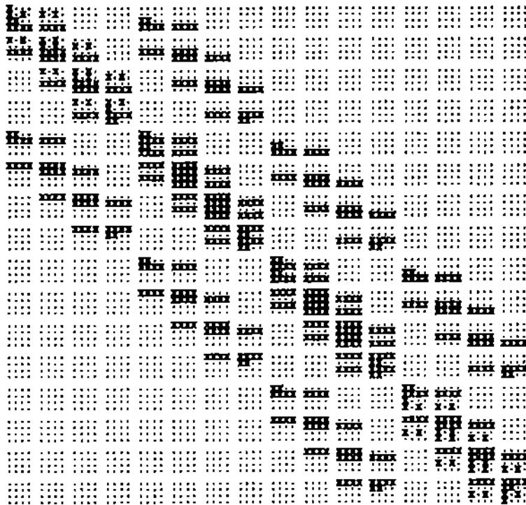
Figure 3: The Intermediate Collocation Matrix for a 4x4 Grid with 64 Unknowns
