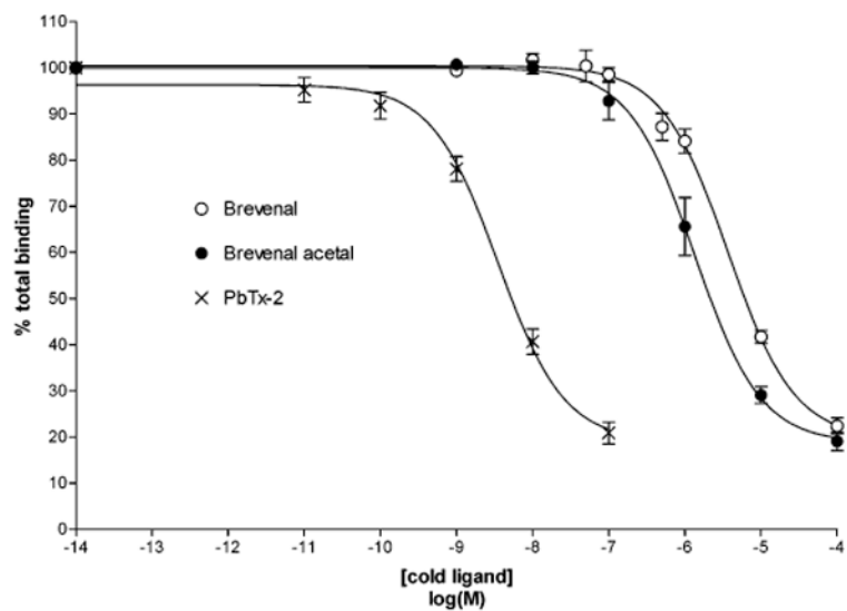
Figure 5. Displacement of tritium-labeled PbTx-3 ( [^3\text{H}]\text{-PbTx-3} ) from rat brain synaptosomes. All values are the mean of at least three experiments, with duplicate determinations at each concentration of competitor in each experiment. Radioactivity associated with the pellet (bound) and the supernatant (free) was determined. A displacement curve for PbTx-2 is provided for reference. Linear regression analysis of each double reciprocal plot yielded r^2 values > 0.98 (data not shown). Convergence of the plots near the ordinate indicates that the interaction between the ligands and [^3\text{H}]\text{-PbTx-3} is competitive.
