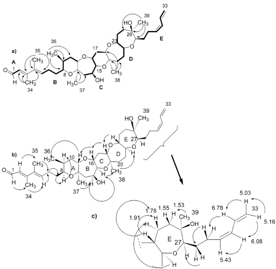
Figure 4. Structure of brevenal determined from NMR data in d_6 -benzene: (a) ^1\text{H} - ^1\text{H} -COSY (bold lines) and HMBC (arrows) correlations, (b) ^1\text{H} - ^1\text{H} -NOESY correlations, (c) detailed view of ring E and side chain from part b.
