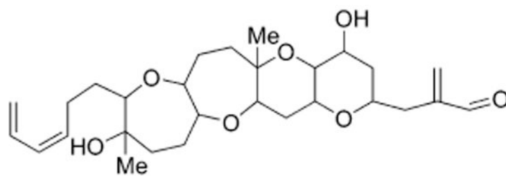
Figure 2. Hemibrevetoxin-B.
