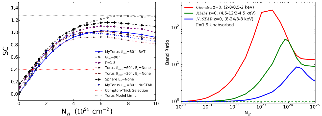
Figure 3. Left: variations in SC with column density based on XSPEC simulations. The blue solid line shows the MYTORUS model used for the SC_{BAT} definition with \Gamma = 1.9 , E_c = 200 keV, and \theta_{inc} = 80^\circ . SC_{NuSTAR} (blue dashed line) only shows small differences from SC_{BAT} ( \Delta SC < 0.07 ) at all column densities. We also show the dependency of SC_{BAT} on inclination angle ( \theta_{inc} , gray circle), intrinsic power law ( \Gamma , purple circle), opening angle with BNTORUS model ( \theta_{open} , pink and brown stars; Brightman & Nandra 2011), or a simple sphere model (black diamonds; Brightman & Nandra 2011). The differences between models are small ( \Delta SC_{BAT} < 0.1 ) except at very high column densities ( N_H > 4 \times 10^{24} \text{ cm}^{-2} ). At very high column densities ( N_H > 4 \times 10^{24} \text{ cm}^{-2} ) the SC measure does not increase at larger column densities. At low column densities ( N_H < 5 \times 10^{23} \text{ cm}^{-2} ), the lack of the high-energy cutoff in the BNTORUS and sphere models raises the SC because of the additional flux in the high-energy emission. A red dotted line shows the Compton-thick lower limit ( SC_{BAT} = 0.4 ) used for this study, and a gray dotted line shows the upper limit from the torus model ( SC_{BAT} = 1.28 ). Right: simulations of obscured sources using band ratios. The band ratio, unlike the SC method, is ineffective at selecting Compton-thick AGNs because of a degeneracy with sources at lower column densities.
