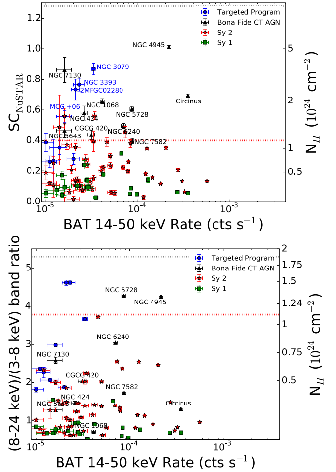
Figure 5. Top: plot of the SC_{\text{NuSTAR}} measurement for nearby ( z < 0.03 ) BAT AGNs. The nine BAT AGNs targeted based on 14–50 keV curvature are shown in blue. Well-known “bona fide” Compton-thick AGNs observed with NuSTAR are shown in black. The simulation limits for an edge-on torus are shown as a gray dotted line, while the lower limit of a Compton-thick column is shown by a red dotted line. Bottom: band ratios of BAT AGNs observed with NuSTAR (8–24 keV/3–8 keV).
