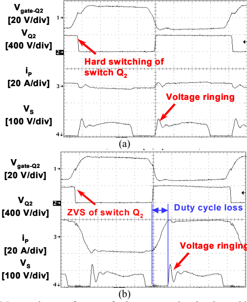
Fig. 8. Measured waveforms of the conventional phase-shifted FB converter at (a) I_o=2 A and (b) I_o=40 A. Time base: 1 \mu s/div.
