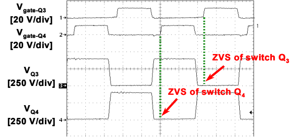
Fig. 10. Measured PWM switch waveforms of the proposed circuit at I_o=2 A. Time base: 2 \mu s/div.
