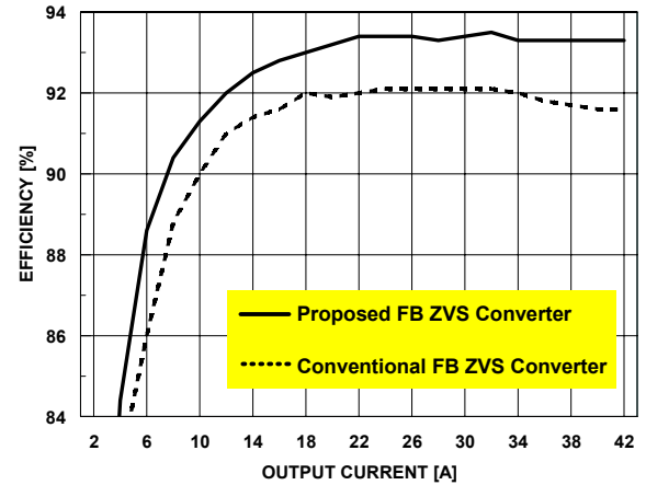
Fig. 7. Measured efficiencies of conventional phase-shifted FB ZVS converter (dashed line) and proposed converter (solid line) as functions of output current.
