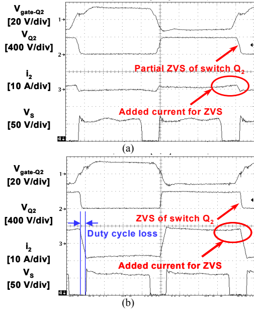
Fig. 9. Measured waveforms of the proposed converter at (a) I_o=2 A and (b) I_o=40 A. Time base: 1 \mu s/div.
