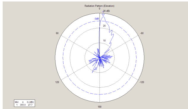
Figure 4.4 Cosecant squared pattern of the antenna
