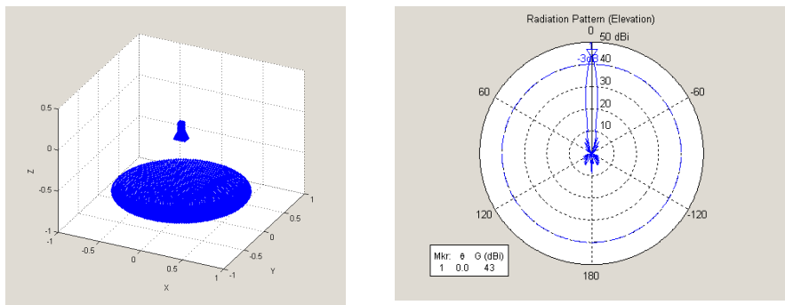
Figure 3.1 A parabolic reflector antenna with pencil beam pattern
