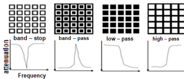
Figure 2.1 Electromagnetic filter behaviors of FSS structures that are differently designed
