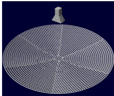
Figure 1.2 A parabolic reflector antenna that has a grid reflector surface
