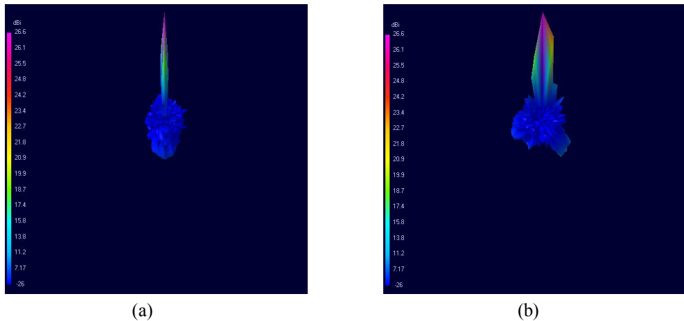
Figure 4.3 (a) Sight of the pattern in Theta: 90 and Phi: 90, (b) Sight of the pattern in Theta: 90 and Phi: 180
