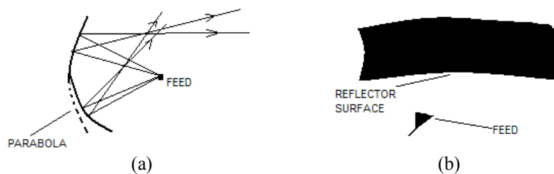
Figure 1.1 (a) Deformation of parabolic reflector to obtain a cosecant squared pattern, (b) A Fan beam antenna
