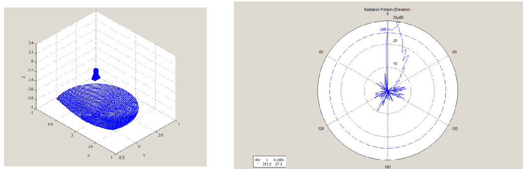
Figure 3.2 An antenna with cosecant squared pattern
