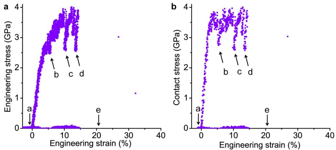
Supplementary Figure S1. Stress-strain curves for FIBed Mo pillars with diameter of 142 nm. (a) Engineering stress (force divided by a fixed cross sectional area) vs. Engineering strain (b) Contact stress (instantaneous force divided by the instantaneous contact area) vs. Engineering strain. Supplementary Figure S1a is reproduced from Figure 2f in the paper.
