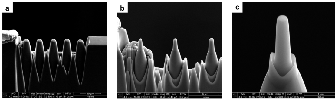
Supplementary Figure S3. Sequential FIB micromachining to obtain nano-sized pillars. (a) Rough machining. (b) Fine processing. (c) Superfine processing.
