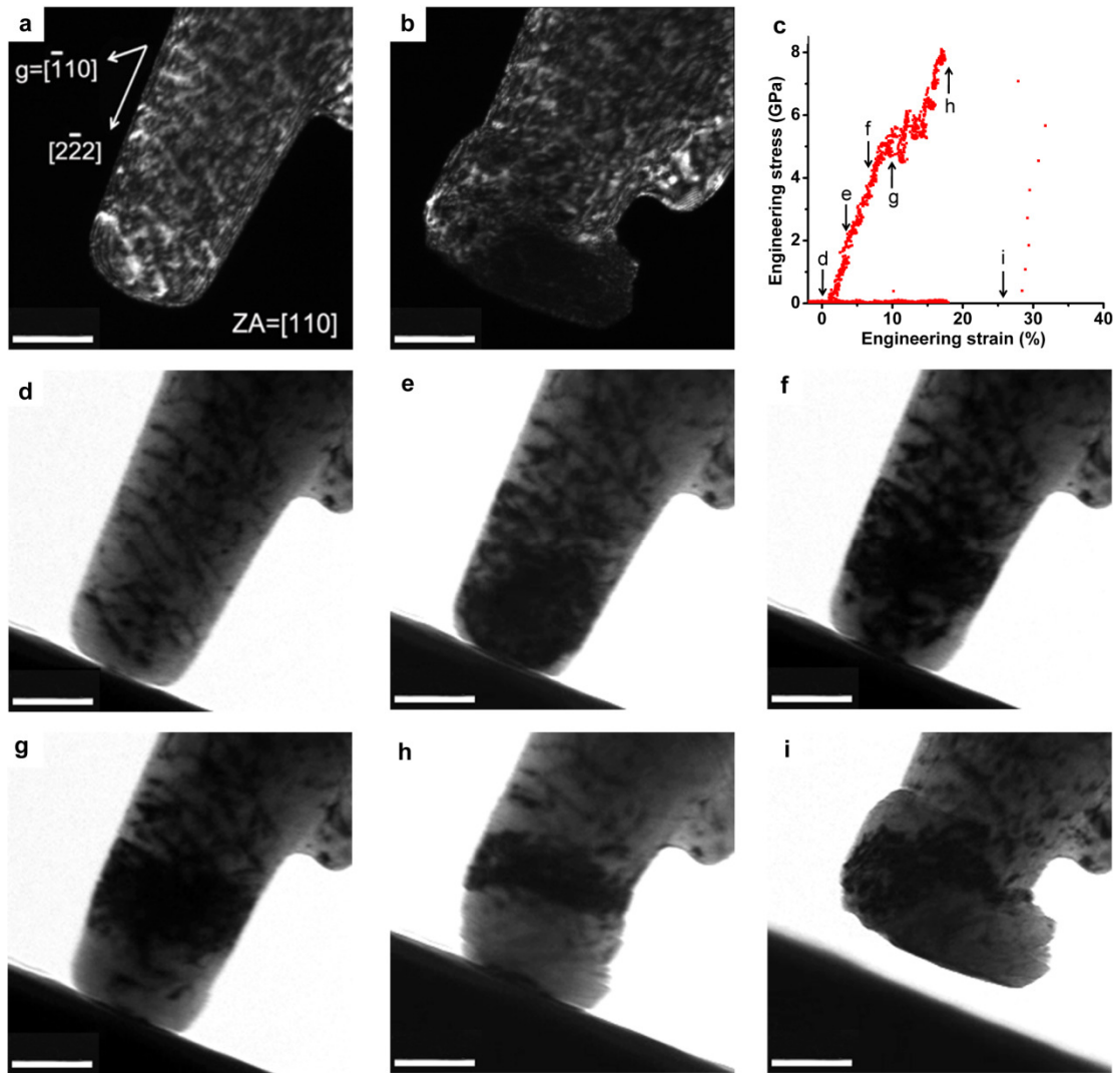
Supplementary Figure S2. In situ compression deformation test of the nanopillar with initial top diameter of 80 nm. Dark field image before (a) and after compression test (b). The corresponding engineering stress vs. strain is shown in (c). (d) through (i) are the still frames extracted from the recorded movies that correspond to the marked points in (c), respectively. The scale bar in each figure represents 50 nm. Obvious dislocation density drop can be observed. The dark contrast shown in the middle of the pillar (g-h) is presumably due to the bending of the pillar.
