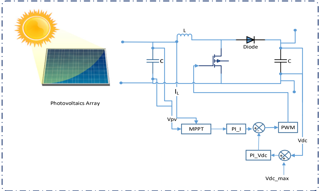
Figure 14. MPPT control of boost converter.
