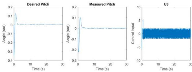
Figure 18. Roll Rotation without Chattering Reduction.
