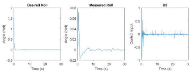
Figure 20. Yaw Rotation without Chattering Reduction.
