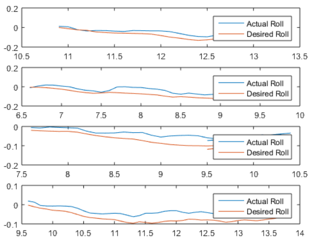
Figure 15. Roll Response for SMC.
