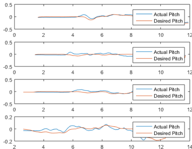
Figure 13. Pitch Response for PID.
