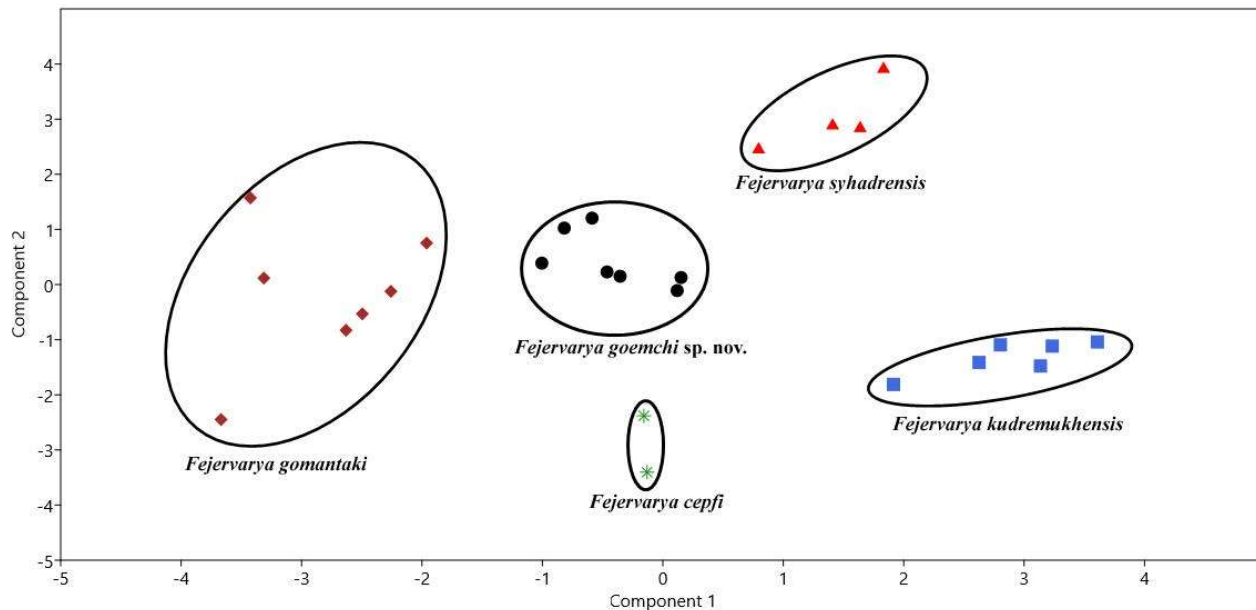
Figure 5. Multivariate Principal Component Analysis for male individuals of 14 morphometric characters marked as * in Table 1 transformed to their ratio to SVL for Fejervarya goemchi sp. nov., F. kudremukhensis , F. cepfi , F. gomantaki and F. syhadrensis .
