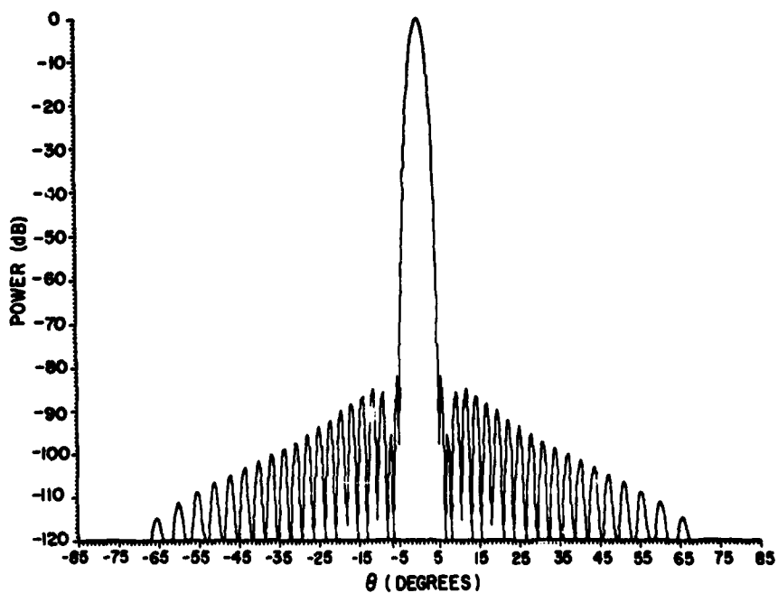
Fig. 10b — Two-way antenna pattern when 45 stationary Hamming-weighted elements spaced \lambda/2 apart are used both on transmit and on receive
