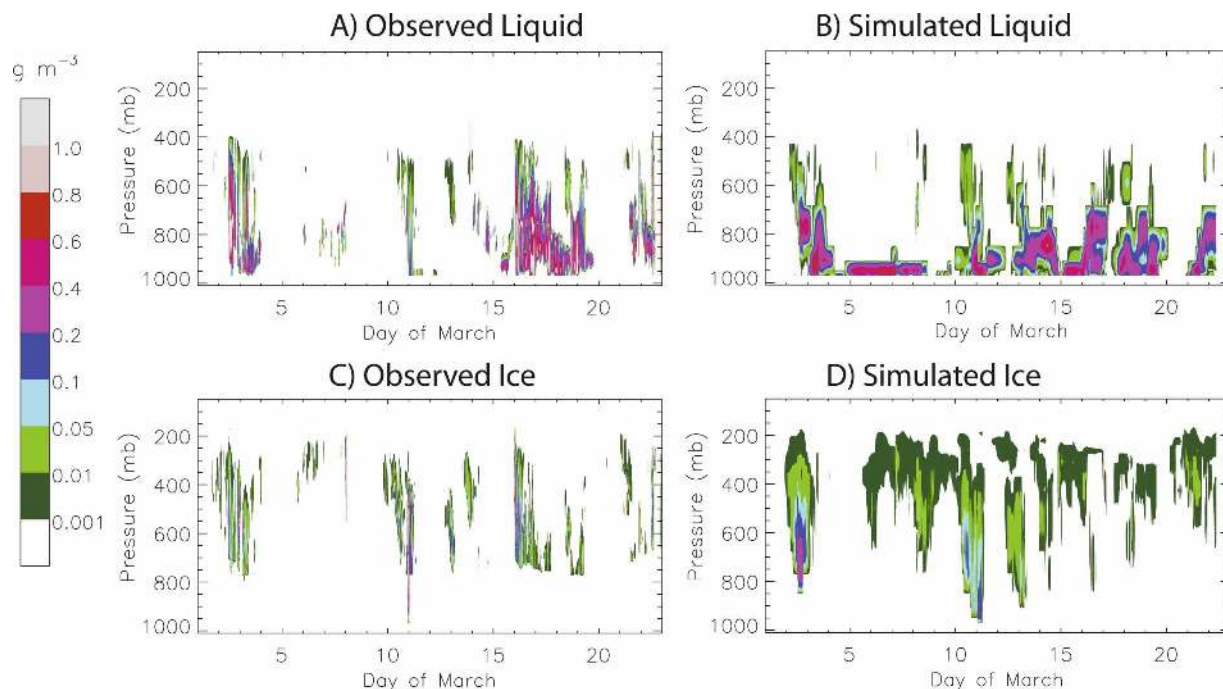
FIG. 1. (a),(c) Observed and (b),(d) simulated (a),(b) LWC and (c),(d) IWC for the March 2000 IOP at the ARM SGP site. Units of \text{g m}^{-3} .
