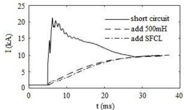
Fig. 8 Bipolar fault current of the \pm 160 kV HVDC system. (a) without current limiting measure; (b) add 500mH current limiting inductor; (c) add the DC SFCL
