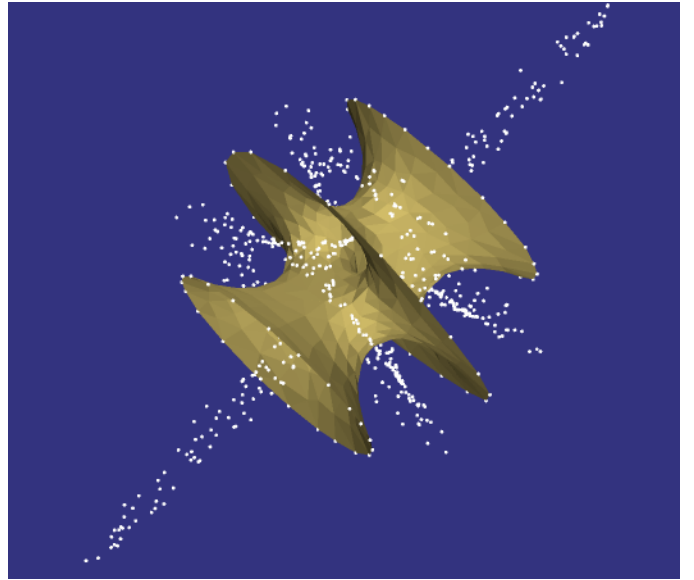
Figure 7. The crust of a set of sample points and the poles (white points) used in its reconstruction. Each sample selects the two vertices of its Voronoi cell that are farthest away, one on either side of the surface, as poles. The poles lie near the medial axis of the surface, sketching planes separating opposite sheets of surface that degenerate to one-dimensional curves where the cross-section of the surface is circular.
