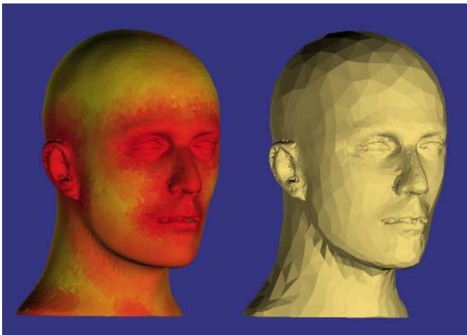
Figure 4. The sampling spacing required to correctly reconstruct a surface is proportional to the distance to the medial axis. On the left is a surface reconstructed from a dense sample. The color represents estimated distance to medial axis—red means close. On the right, we use the estimated distance to thin the data to a .5-sample (meaning that the distance to the nearest sample for any point on the surface is at most half the distance to the medial axis), and then reconstruct. There were about 12K samples on the left and about 3K on the right.
