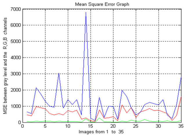
Figure 3: MSE measurements between the R, G, B components and the grayscale version for 35 images.
