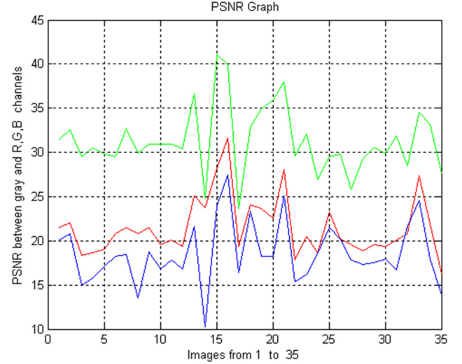
Figure 6: PSNR measurements between R, G, B components and grayscale version for 35 color images.
