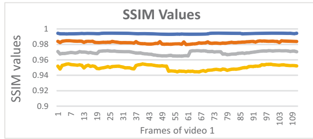
Figure 11: SSIM values of video 1.
