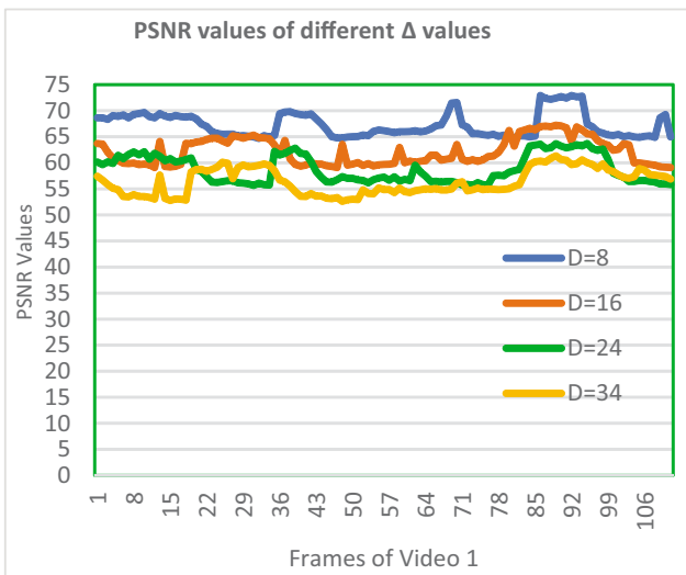
Figure 10: PSNR values for watermarked video 1.
