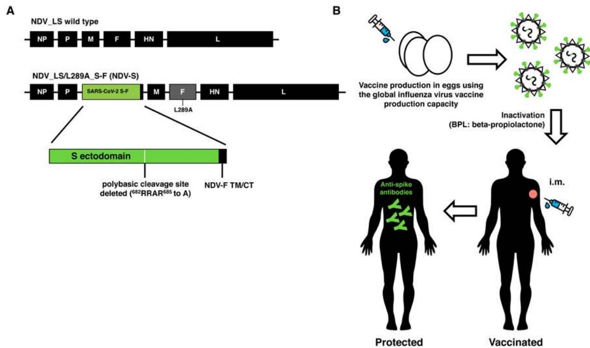
Figure 1. Design and concept of an inactivated Newcastle disease virus (NDV)-based severe acute respiratory syndrome coronavirus 2 (SARS-CoV-2) vaccine. (A) Design of the NDV-S vaccine. The sequence of the spike-fusion (S-F) chimera (green: ectodomain of S, and black: the transmembrane domain and cytoplasmic tail of the NDV F protein) was inserted between the P and M gene of the NDV LaSota (NDV_LS) strain L289A mutant (NDV_LS/L289A). NDV-S: NDV_LS/L289A_S-F. The polybasic cleavage site of the S was removed ( ^{682}RRAR^{685} to A). (B) The concept overview of an inactivated NDV-based SARS-CoV-2 vaccine. The NDV-S vaccine could be produced using the current global influenza virus vaccine production capacity. Such an NDV-S vaccine displays abundant S proteins on the surface of the virions. The NDV-S vaccine could be inactivated by beta-propiolactone (BPL). The NDV-S vaccine could be administered intramuscularly (i.m.) to elicit protective antibody responses in humans.
