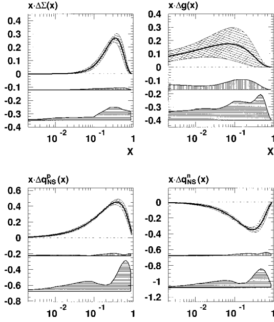
FIG. 5. Polarized parton distribution functions determined from the PQCD analysis at Q_i^2=1 GeV 2 . Their statistical uncertainty as obtained from the QCD fit is shown by a band with crossed hatch. The experimental systematic uncertainty is indicated by the vertically hatched band, and the theoretical uncertainty by the horizontally hatched band.
