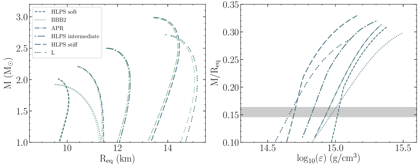
Figure 5. Left panel: effect of spin on the mass versus equatorial radius curves for six representative EOS allowing for a wide range of stiffness. Two curves with dark and light lines are shown for each EOS. For each pair, the lighter curve with smaller radii corresponds to the zero-spin mass-radius curve, while the darker curve with larger radii is the mass-radius curve for stars spinning at 205 Hz. The EOS in order of increasing stiffness (i.e., in order of increasing radius for a 1.4 M_{\odot} star) are HLPS Soft (Hebeler et al. 2013), one of the softest EOS allowed by nuclear physics; BBB2 (Baldo et al. 1997) is a soft EOS just marginally ruled out by the observation of a 1.97 M_{\odot} pulsar; APR (Akmal et al. 1998) includes boost corrections; HLPS Intermediate and Stiff are representative EOS from Hebeler et al. (2013); and L (Pandharipande & Smith 1975), a very stiff EOS, is most likely ruled out by the Laser Interferometer Gravitational-Wave Observatory (LIGO) observation of GW170817 (Abbott et al. 2017). The HLPS EOS are also shown in Figures 1 and 2. Right panel: effect of spin on the equatorial compactness ratio M/R versus central energy density. The order of curves from left to right at a value of M/R_{\text{eq}} = 0.15 is from stiffest to softest EOS. Two curves, corresponding to 0 and 205 Hz are plotted for each EOS, however the difference between the curves is smaller than the line width so it is difficult to see the difference by eye. The gray horizontal box shows the compactness range of M/R_{\text{eq}} = 0.156^{+0.008}_{-0.010} for the ST+PST model reported in Riley et al. (2019).
