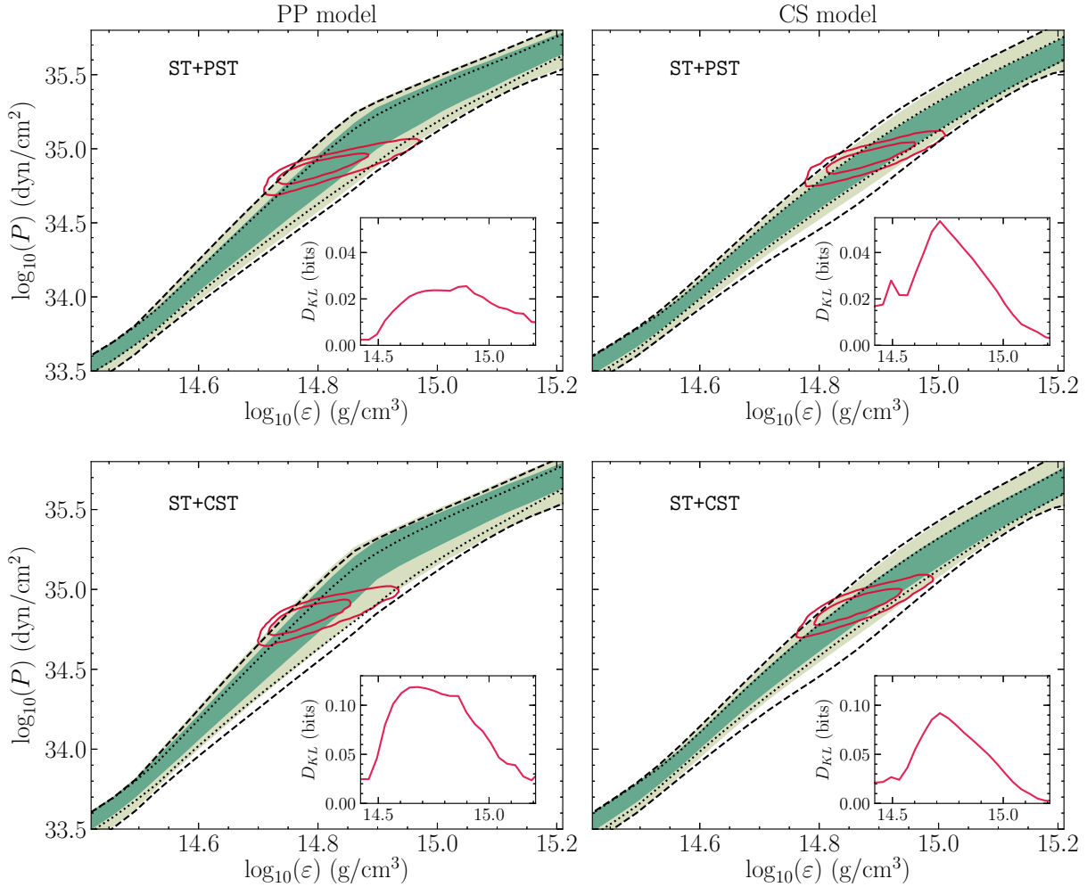
Figure 2. Marginal posterior distributions of the pressure P conditional on energy density \varepsilon , p(P|\varepsilon, \mathbf{d}, \mathcal{M}) , for the PP model (left) and the CS model (right), and for both the preferred ST+PST model (upper panels) and the alternative ST+CST model (lower panels). At each value of \varepsilon , there exist 68% and 95% posterior credible intervals for the pressure P ; we connect these intervals to form the shaded bands. The black dotted and dashed lines respectively indicate the joined 68% and 95% credible interval bands, but for the conditional and marginal prior distribution, p(P|\varepsilon, \mathcal{M}) . The red contours in each panel indicate the 68% and 95% highest-density posterior credible regions of central energy density and central pressure. Constraints on the EOS for densities higher than these contours are only determined by our choice of parameterization and are not directly informed by the mass-radius likelihood function (and thus in turn, the data). The lower-right inset panels illustrate the evolution of the Kullback-Leibler (KL) divergence with respect to the energy density, showing that most posterior information is gained for densities below 10^{15} \text{ g cm}^{-3} , not coincidentally the highest possible central density reached in PSR J0030+0451. Note that due to finite sampling noise the precise features of the evolution of the KL divergence might be disputed, but the global trend of the curve is unaffected.
